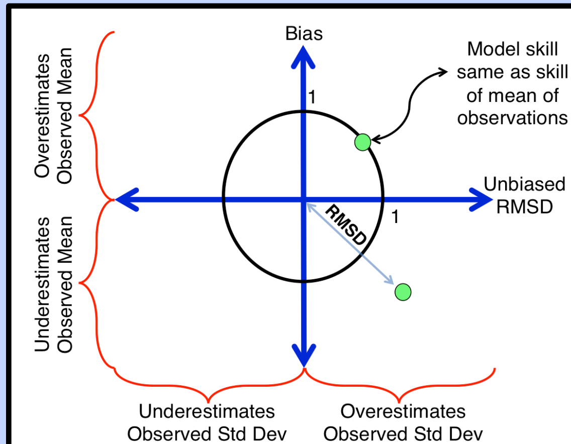
Figure 3. Target Diagram analysis: the total root mean square difference (RMSD) between the observations and the model results, normalized by the standard deviation of the observations. (Jolliff et al., 2009, JMS, doi10.1016/j.jmarsys.2008.05.014).
