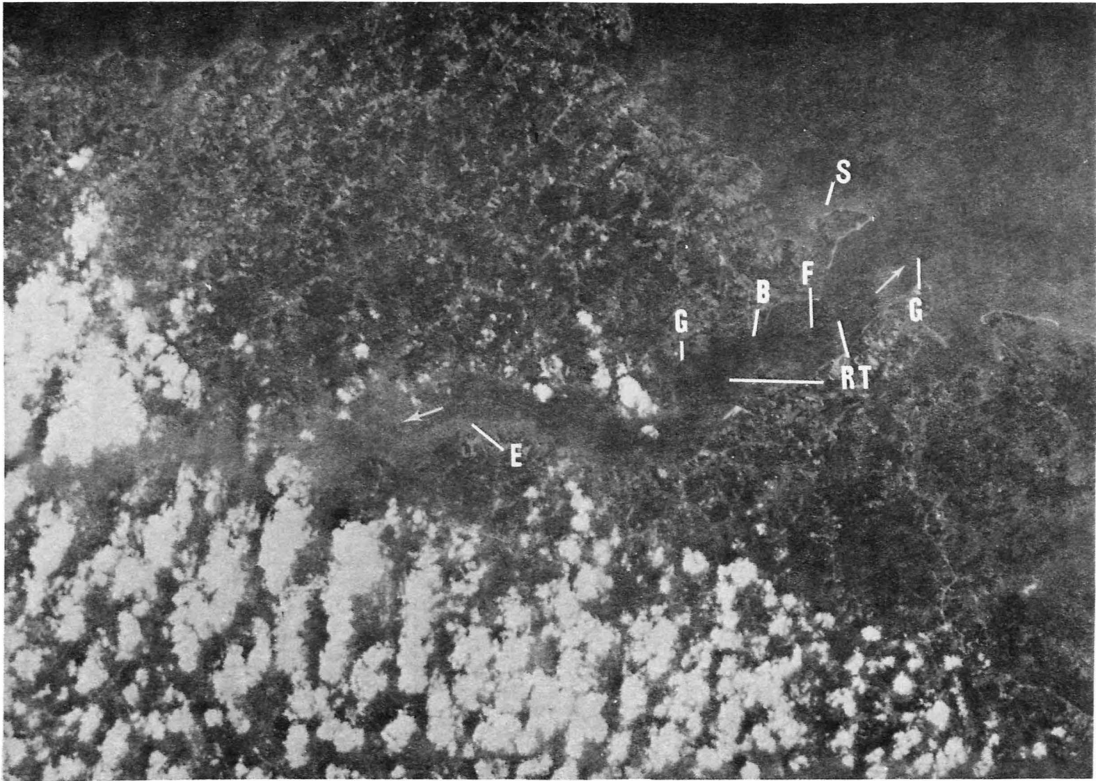
Figure 18. Skylab 3 natural color photograph of the Rappahannock Estuary, Sept. 12, 1973. For explanation of letter annotations, see text.
