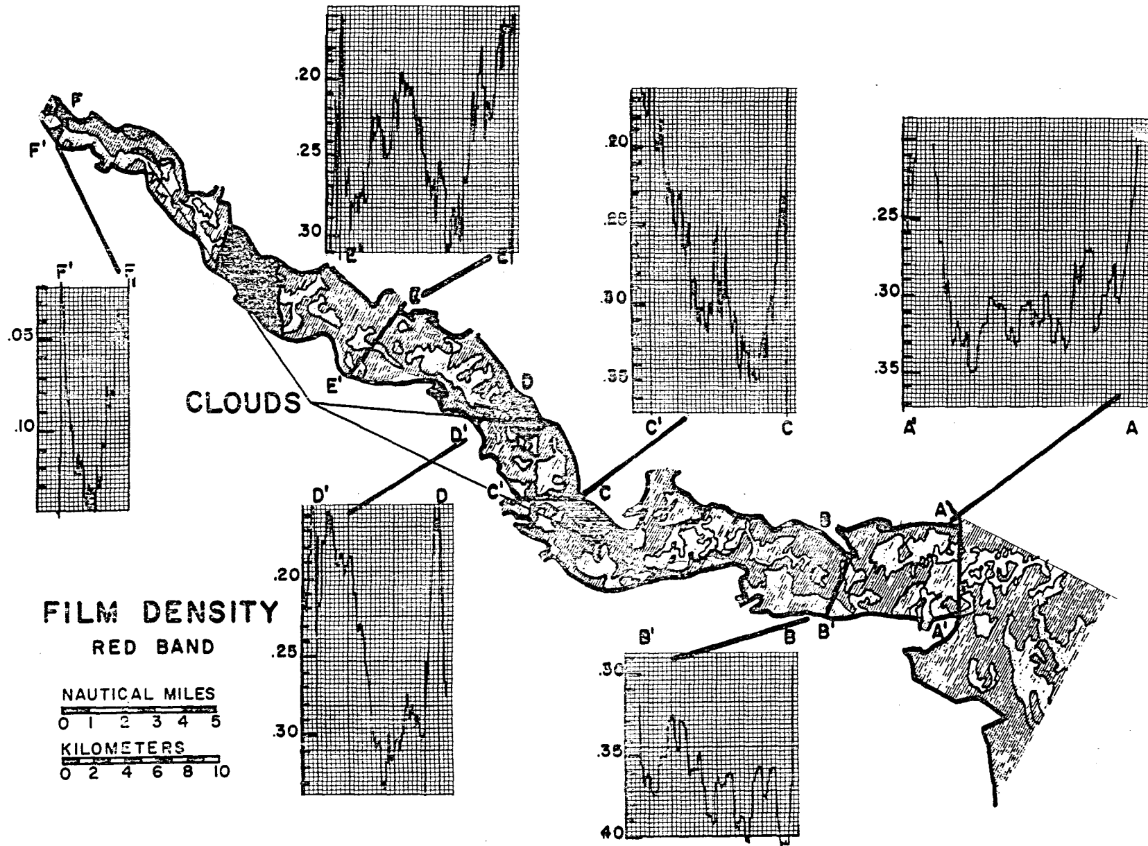
Figure 22. Water color distributions and cross profiles of the Rappahannock Estuary, Sept. 12, 1973, derived from red band film density plots of a Joyce-Loebl microdensitometer.
