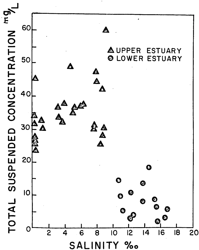
Figure 26. Scatter plot of total suspended material (sediment) versus salinity. From surface truth observations, Sept. 12, 1973 (Rappahannock Estuary).
