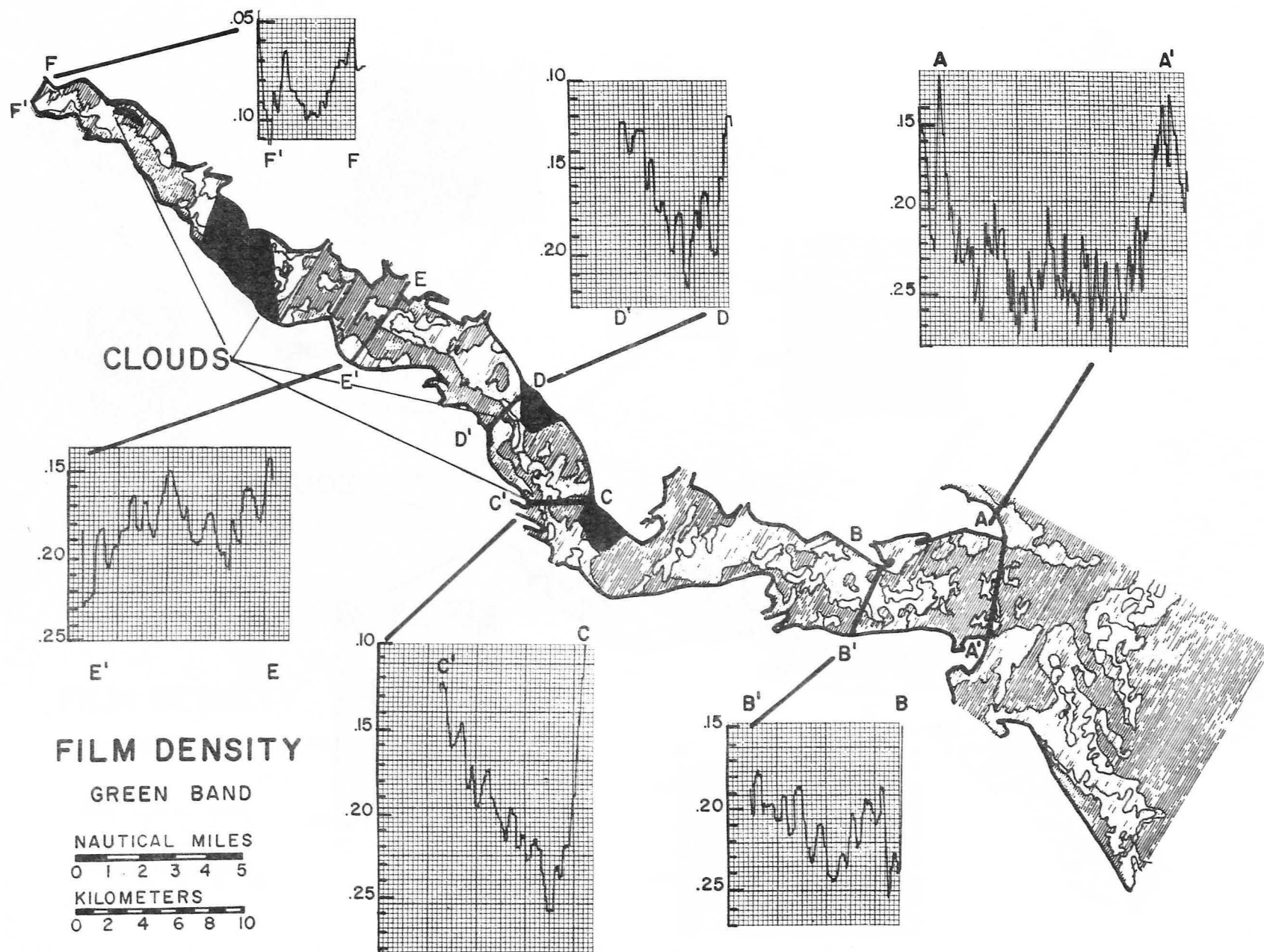
Figure 23. Water color distributions and cross profiles of the Rappahannock Estuary, Sept. 12, 1973, derived from green band film density plots of a Joyce-Loebl microdensitometer.
