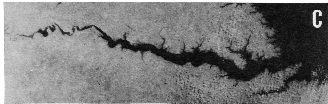
Figure 17. Reproductions of Skylab 2 imagery of the Rappahannock test site, June 12, 1973. A - red band; B - green band and C - black and white infrared. For explanation of letters, see text.
