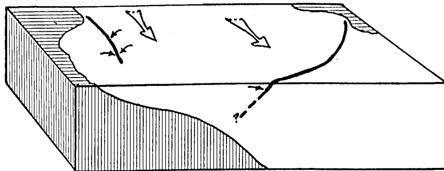
Figure 7. Schematic diagrams of different boundary types in relation to bottom geometry, configuration and secondary currents, single arrows; predominate tidal flow, double arrows.
