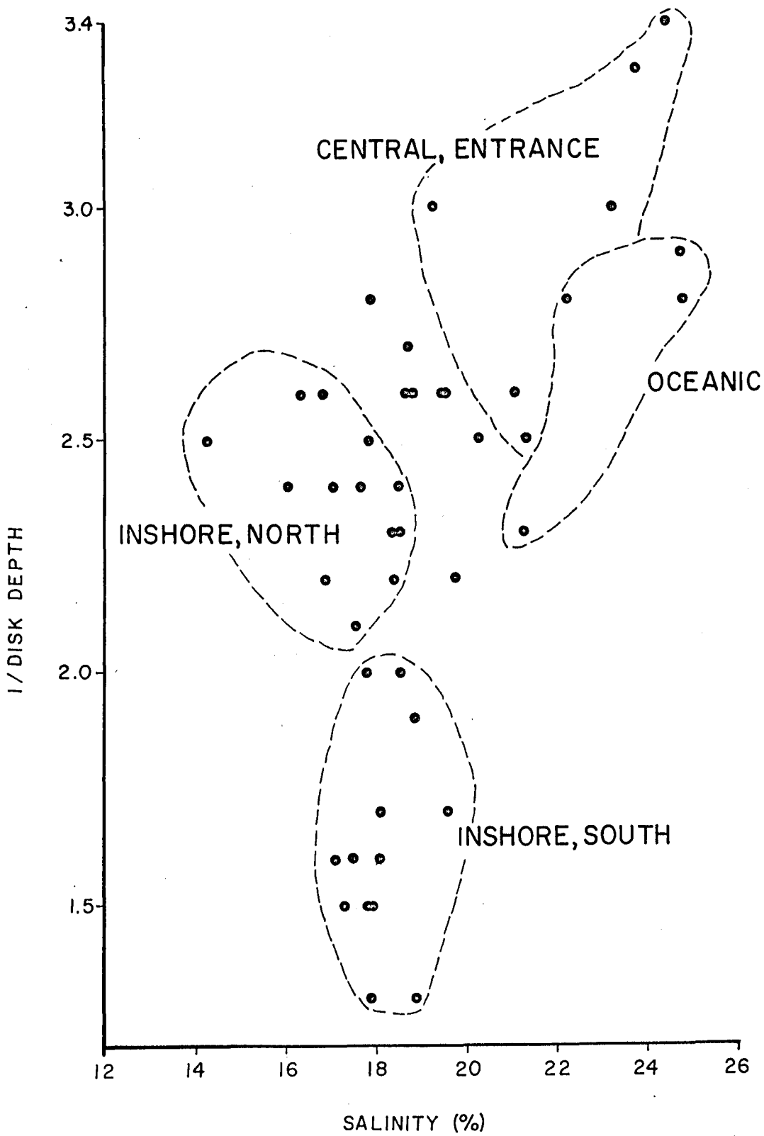
Figure 10. Scatter diagrams of 1/disk depth versus salinity for stations in lower Chesapeake Bay. May 31, 1973. Clusters define different water masses.
