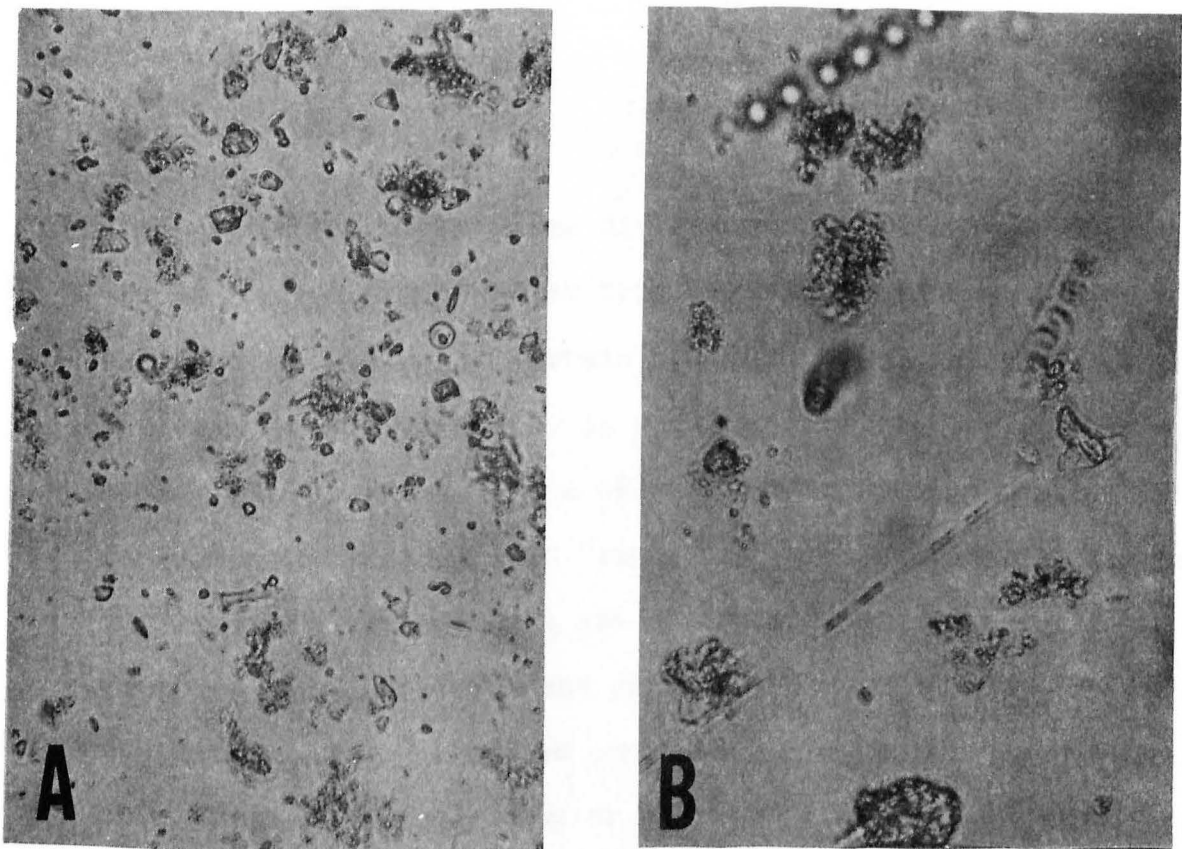
Figure 1. Microphotographs of light scattering suspended material common to the Rappahannock Estuary; A, mainly sediment particles and debris from the upper estuary; B, mainly phytoplankton from the lower estuary.
