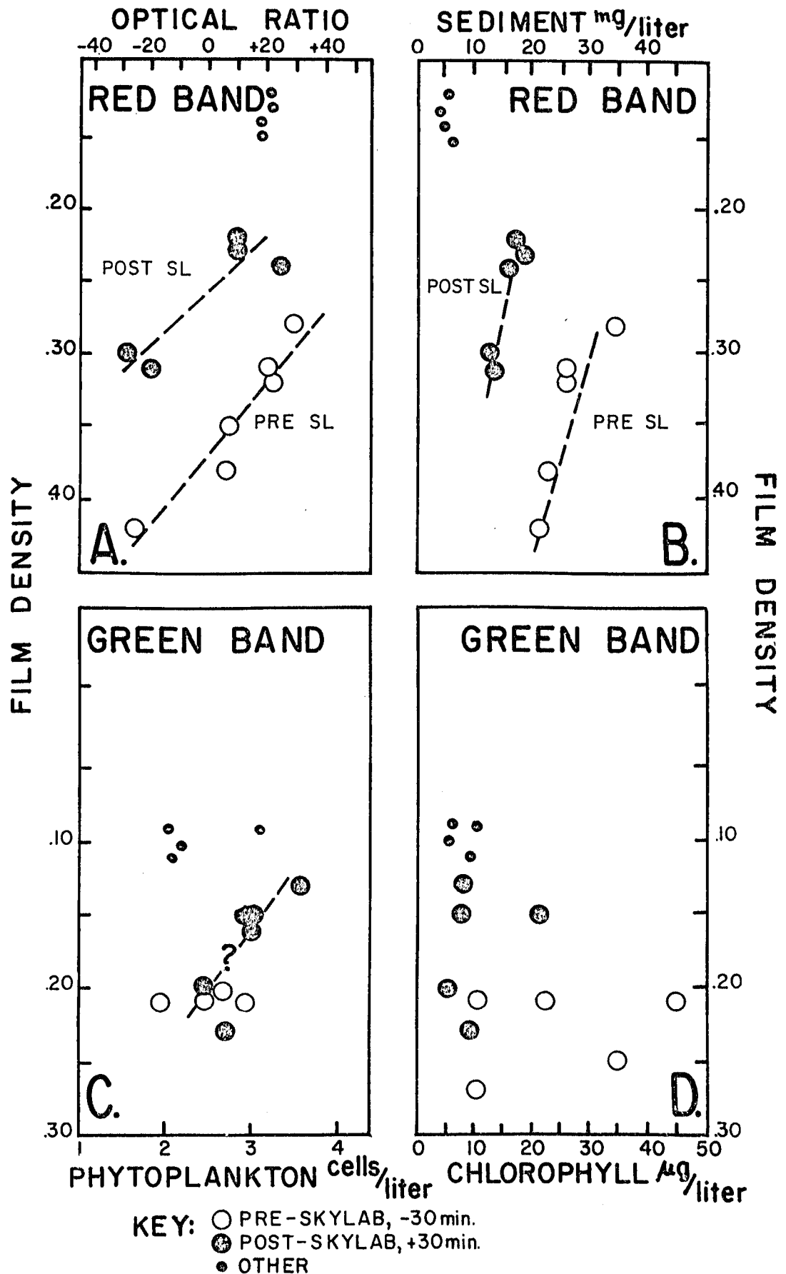
Figure 30. Relationships of film density derived from the Joyce-Loebl microdensitometer in red and green bands to A. Optical ratio, B. Sediment (total suspended material), C. Phytoplankton, D. Chlorophyll. From Skylab 3 observations, Sept. 12, 1973.
