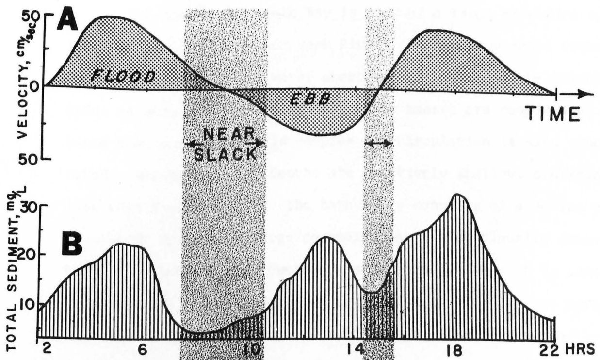
Figure 2. Time variations of current velocity (A) in relation to corresponding variations of total suspended material (B) in the upper Rappahannock Estuary.
