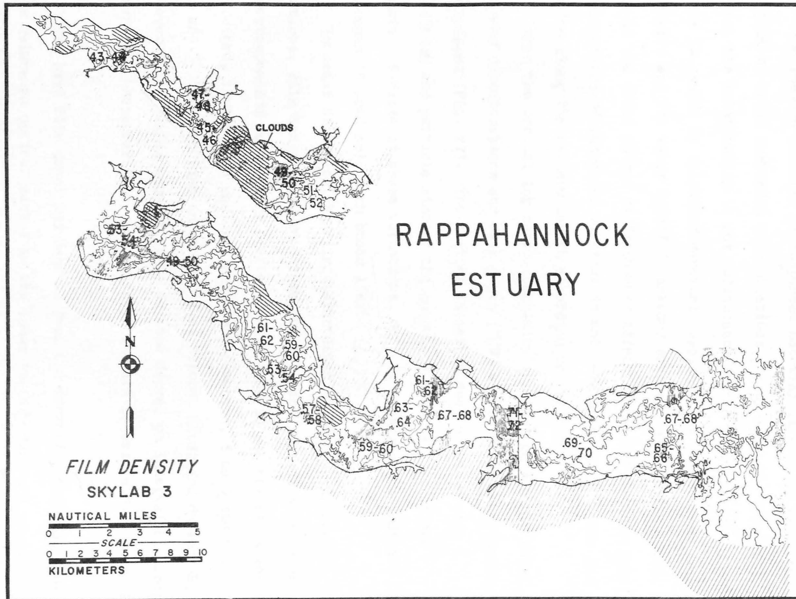
Figure 25. Water color distributions of the Rappahannock Estuary Sept. 12, 1973 derived from film density plots of natural color film in a Joyce-Leobl microdensitometer. Values are film density units.
