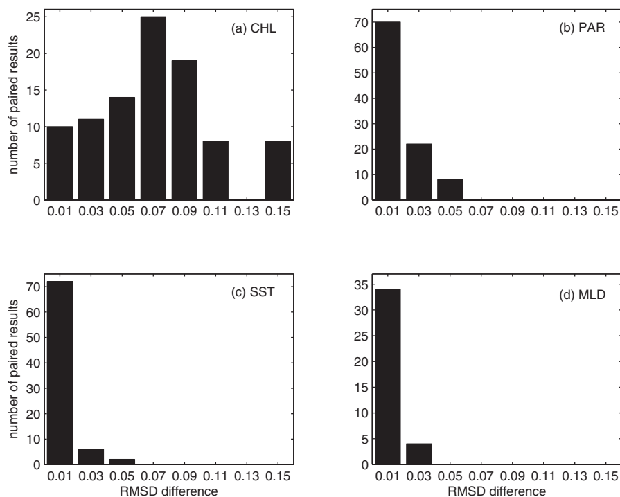
Figure 4. Difference in RMSD of \log\text{NPP}_{N=85} between paired results available for each participating model when only one of the input variables was from an alternate source: (a) chlorophyll (CHL) (24 models), (b) PAR (30 models), (c) SST (16 models), and (d) MLD (5 models).
