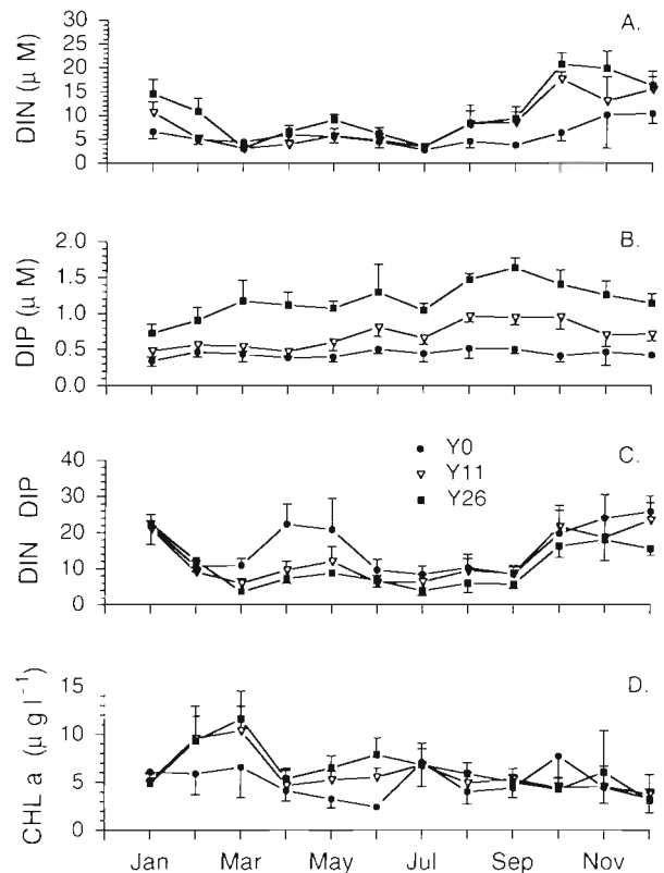
Fig. 4. Mean monthly (A) dissolved inorganic nitrogen (DIN), (B) dissolved inorganic phosphorus (DIP), (C) DIN:DIP ratios, (D) chlorophyll a at Y0, Y11, and Y26 for the period of January 1985 to December 1987. Bars are 1 SE
