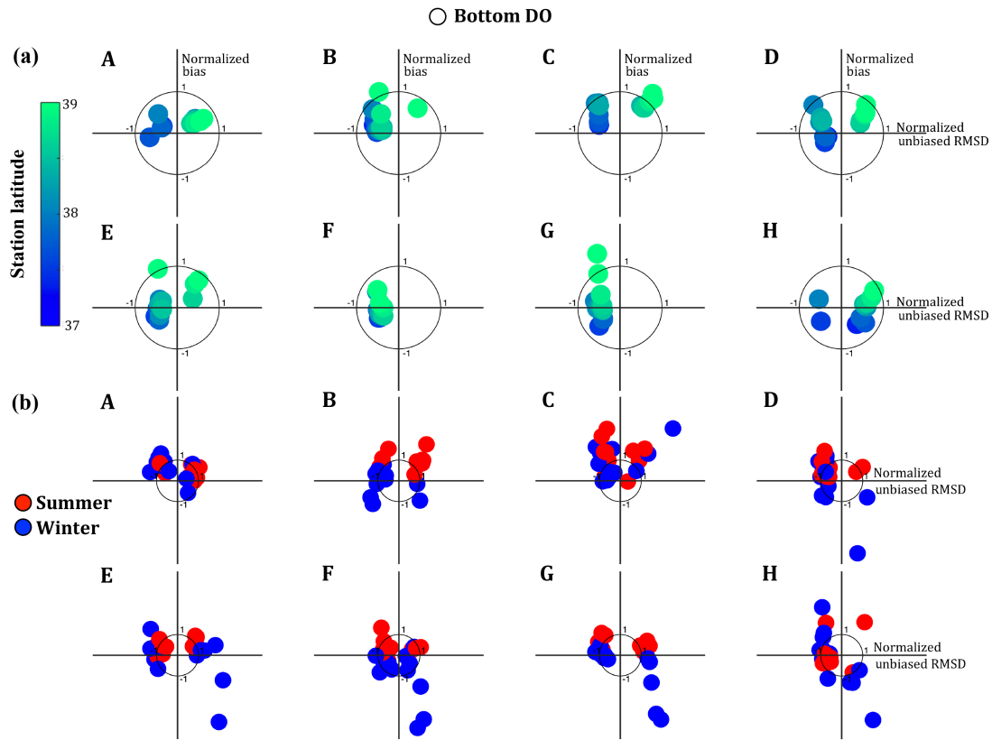
Figure 5. Normalized target diagrams for Models A–H demonstrating the (a) temporal and (b) spatial skill in resolving the variability of bottom dissolved oxygen concentrations. In (a) the individual dots represent the 13 stations along the main stem of the Chesapeake Bay. In (b) the dots represent the 24 months of 2004–2005 and are delineated by color: red is summer (May–September) and blue is winter (October–April).
