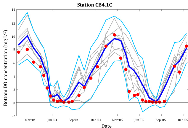
Figure 9. Time series of bottom dissolved concentrations for station CB4.1C. Red dots represent the 34 observations made during 2004–2005. Grey lines are the individual model simulations. The dark blue line represents the Model Mean while the cyan line represents the 95 % confidence interval of the model simulations.
