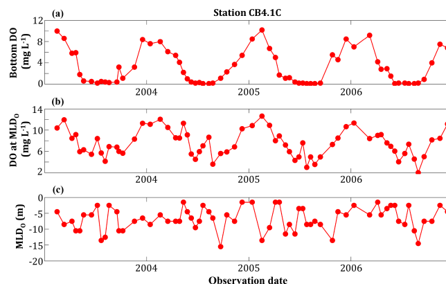
Figure 11. Time series of observations at station CB4.1C from 2003 to 2006 for (a) bottom dissolved oxygen, (b) dissolved oxygen at the MLD_O , and (c) MLD_O .
