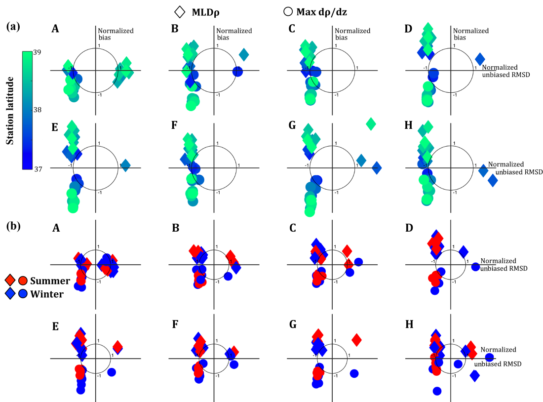
Figure 7. Normalized target diagrams for Models A–H demonstrating the (a) temporal and (b) spatial skill in resolving the variability of the strength of density stratification (circles) and the depth of pycnocline initiation (diamonds). In (a) the individual dots represent the 13 stations along the main stem of the Chesapeake Bay. In (b) the dots represent the 24 months of 2004–2005 and are delineated by color: red is summer (May–September) and blue is winter (October–April).
