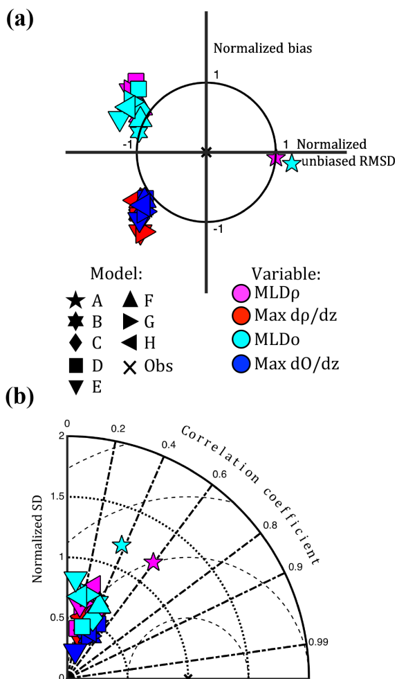
Figure 6. Normalized summary (a) target and (b) Taylor diagram illustrating model skill of MLD ρ and MLD O , max dρ/dz, and max dO/dz at 13 Chesapeake Bay stations for 2004–2005. The “x” represents the skill of a model that perfectly reproduces the observations. Since RMSD of stratification is only computed at stations where both the observations and model exhibit stratification, the Model Mean is not calculable for these variables.
