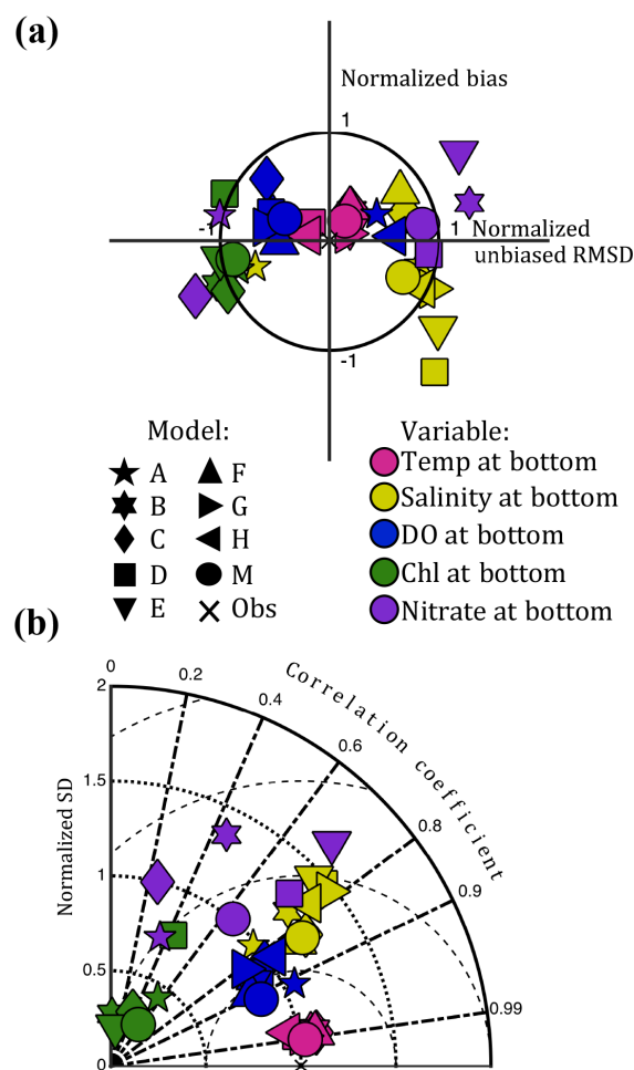
Figure 8. Normalized summary (a) target and (b) Taylor diagram illustrating model skill of bottom temperature, salinity, chlorophyll, nitrate, and dissolved oxygen at 13 Chesapeake Bay stations for 2004–2005. The “x” represents the skill of a model that perfectly reproduces the observations.
