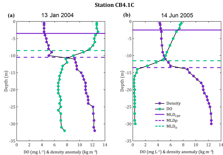
Figure 3. Density and dissolved oxygen profiles for a mid-bay station (CB4.1C) on (a) 13 January 2004 and (b) 14 June 2005, comparing the 0.1 \text{ kg m}^{-4} stratification definition used by the CBP ( \text{MLD}_{\text{CBP}} ) with the 10 % threshold definitions used here for density ( \text{MLD}_{\rho} ) and oxygen ( \text{MLD}_{\text{O}} ).
