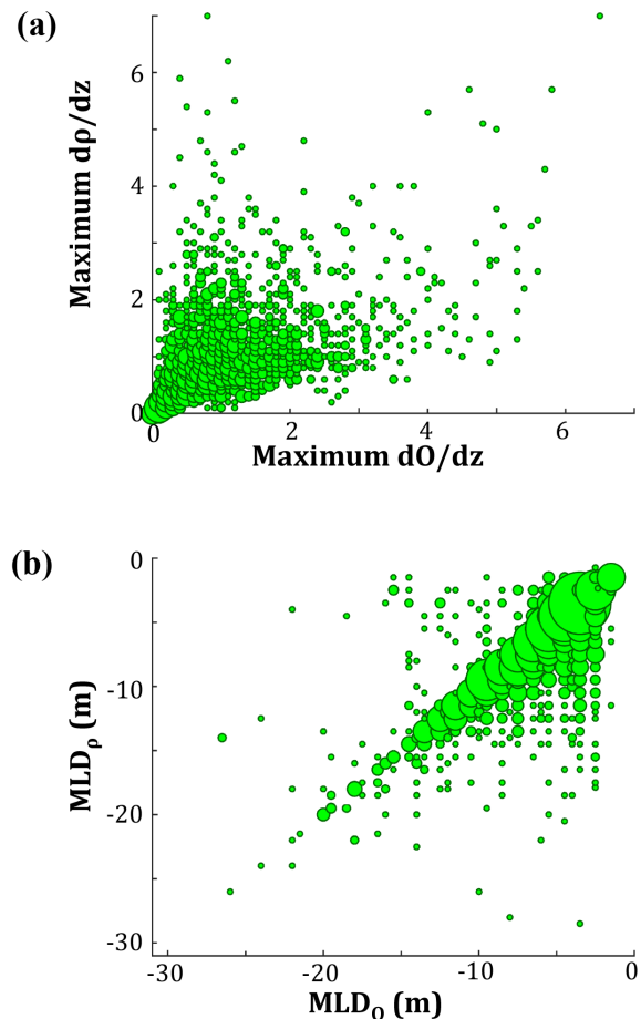
Figure 10. Scatter plots comparing observations of (a) the strengths of stratification of the pycnocline and oxycline and (b) the oxygen- and density-defined mixed layer depths. Size of the circles is proportional to the number of observations. Observations are from 1998 to 2006 at the 13 Chesapeake Bay stations shown in Fig. 2.
