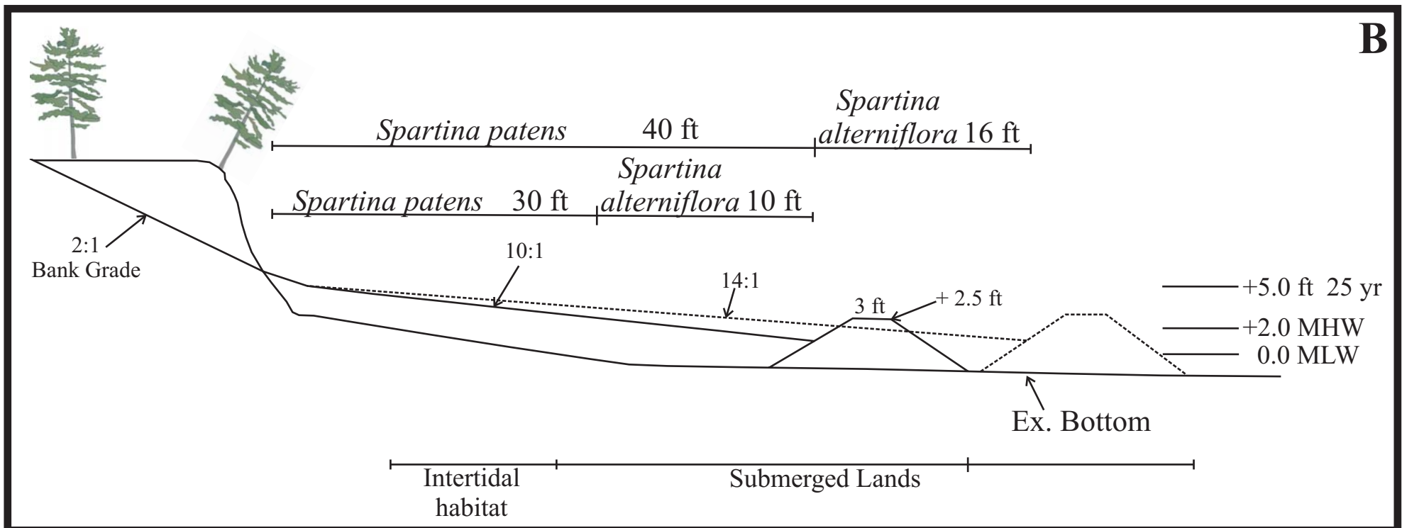
Figure 26. A) Shore protection options with encroachment, level of protection, and habitat value. B) Two sill options showing the amount of encroachment and the amount of habitat gained.
