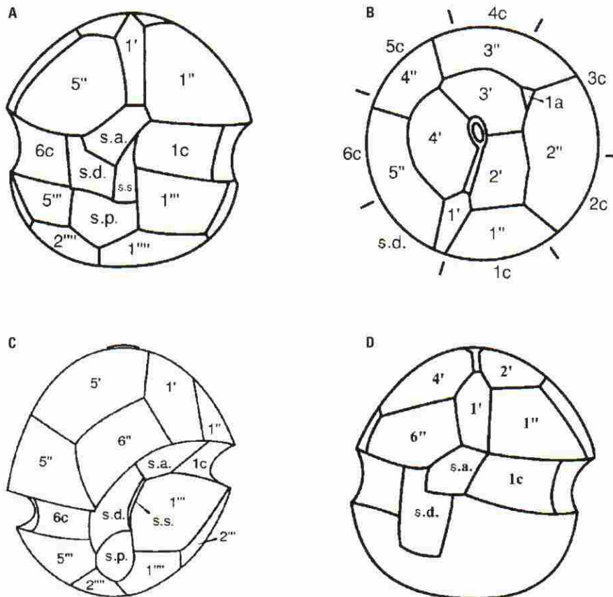
Figure 2. Schematic illustrations of Pfiesteria and Pfiesteria -like dinoflagellate. These four panels show how the epithecal plates fit together and how they are labeled. (A) Ventral view of P. piscicida . (B) Apical view of P. piscicida . (C) Ventral view of cryptoperidiniopsisoid. (D) Ventral view of the epithea of "Lucy."
