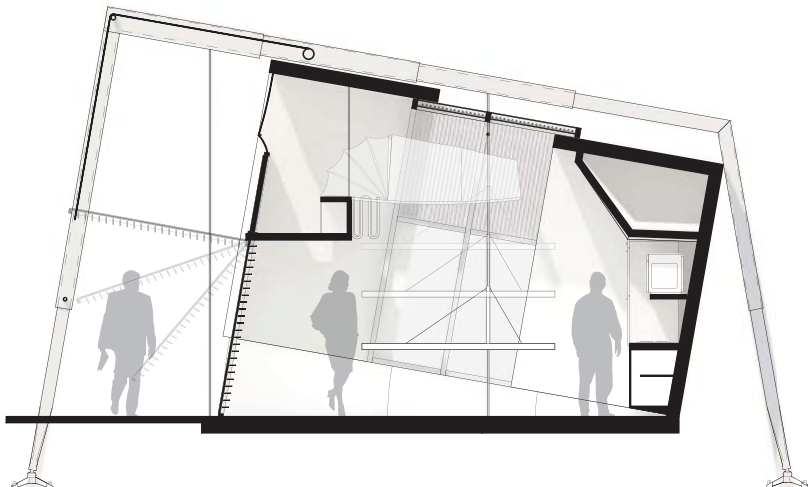
Section E-E
