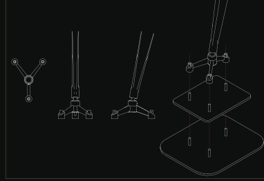
Adjustable Foot
