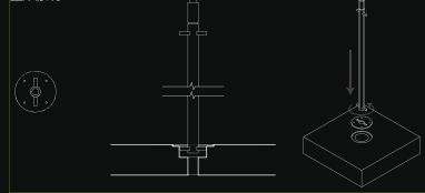
Tension Rod Connection
