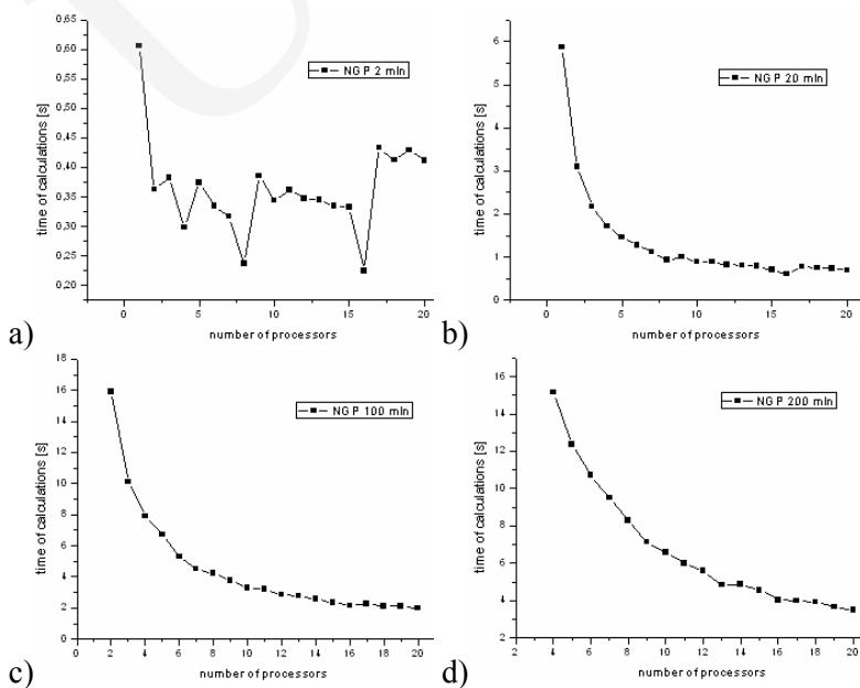
Fig. 8. Time of charge density calculations versus the number of processors used for the parallel run, using the NGP method and a different number of macro particles: a) 2 mln, b) 20 mln, c) 100 mln, d) 200 mln
