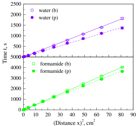
Fig. 4. Penetration time vs. the square of the distance for water and formamide on the bare (b) and precontacted (p) silica gel layers on the glass plates.
