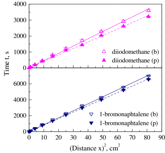
Fig. 3. Penetration time vs. the square of the distance for diiodomethane and 1-bromonaphthalene on the bare (b) and precontacted (p) silica gel layers on the glass plates.
