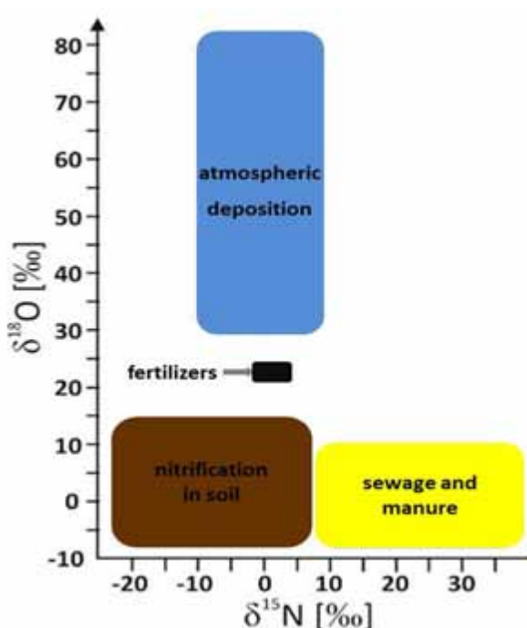
Figure 8: Ranges of isotopic compositions for major nitrate sources (based on Mayer et al., 2002; Mayer 2005).
