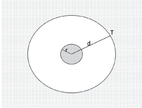
Figure 3: Density of DQV in the centre, on the surface and distant from a stellar object.
