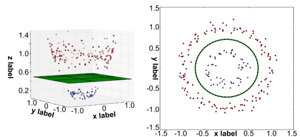
Figure 3: Once the data is mapped to a higher dimension, we find a hyperplane to separate it [4].
