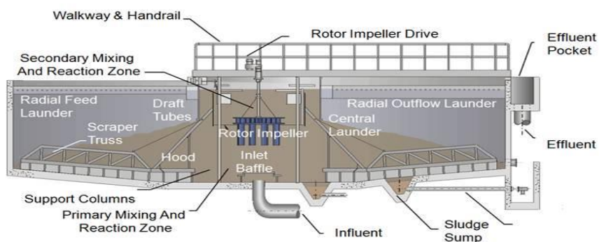
Figure 2.1.) Solids-Contact Clarification System - IS Accelerator by Degremont Technologies
