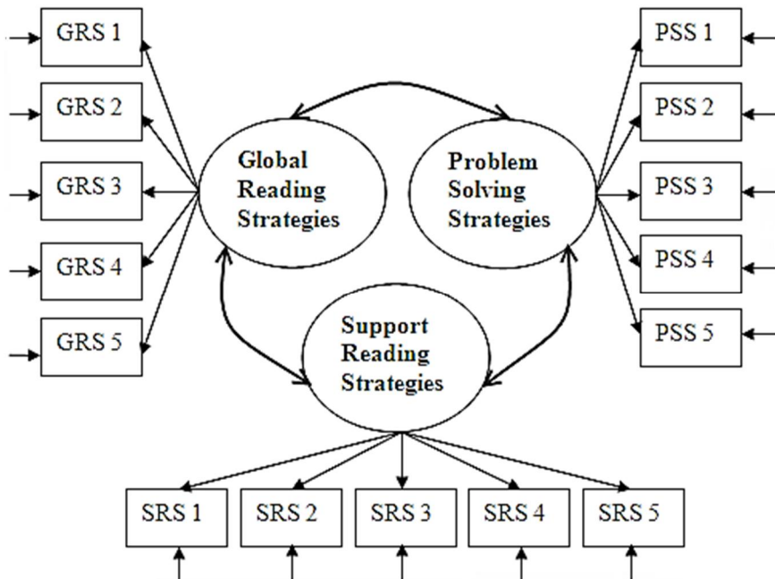
Figure 1 Baseline CFA model for MARSII-R
