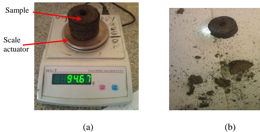
Figure 5 Set-up during shatter index test (a) Weighing of sample before test (b) Shattered sample after the test
