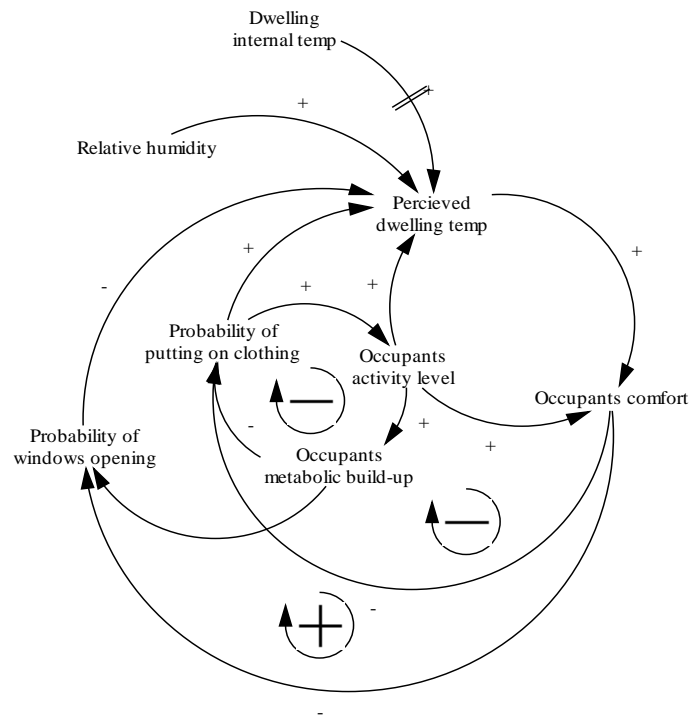
Figure 4. CLD for occupants' thermal comfort module
