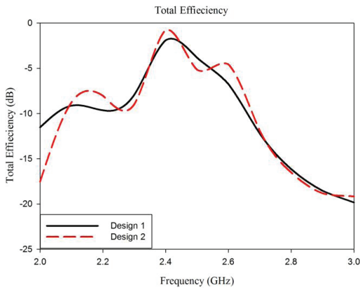
Figure 13: The comparison of total efficiency for Design 1 and Design 2
