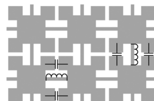
Figure 6: The UC structures are designed to have connectivity with the equivalent circuit introduced
