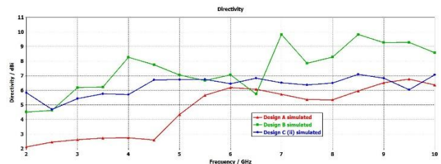
Figure 11: Directivity of all the simulated results
