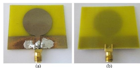
Figure 2: The (a) front and (b) back view of fabricated Design A
