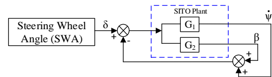
Figure 3: Block Diagram of Closed-Loop System
