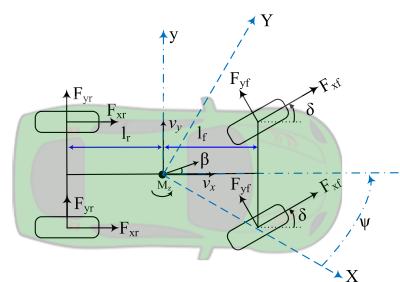
Figure 2: Planar Vehicle Dynamic
