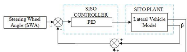
Figure 1: Block Diagram of Overall System
