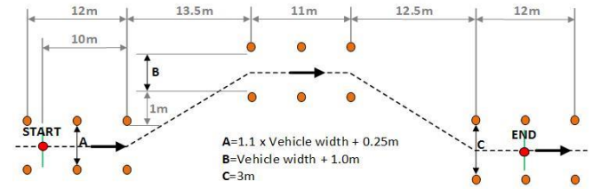
Figure 4: ISO 3888-2 Double Lane Change Test Track
