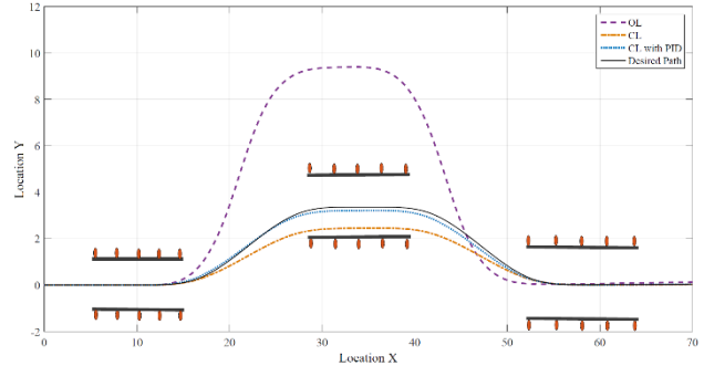
Figure 7: Vehicle Trajectory for Double Lane Change at Constant Speed, 40km/h
