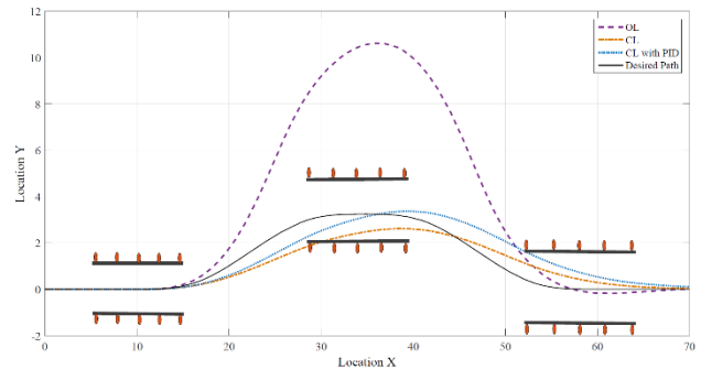
Figure 8: Vehicle Trajectory for Double Lane Change at Constant Speed, 90km/h
