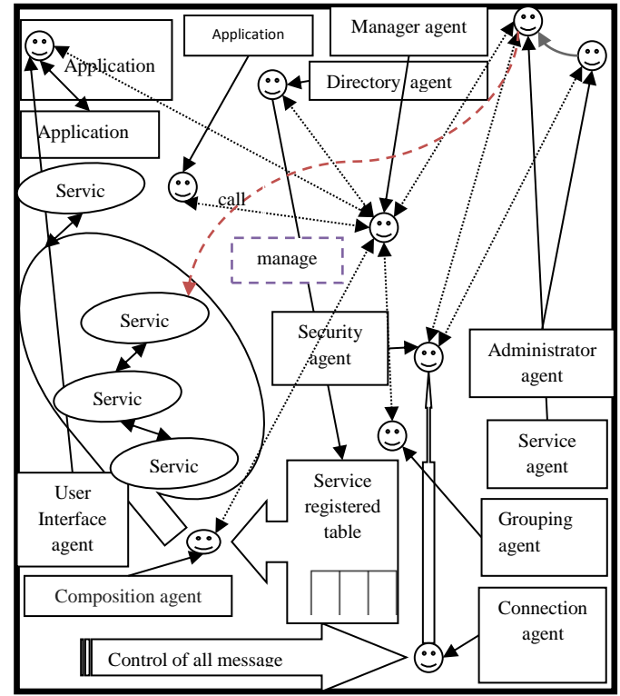
Figure 6: Proposed Model
