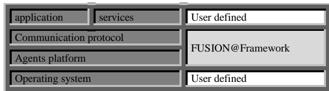
Figure 1: FUSION framework [38]
