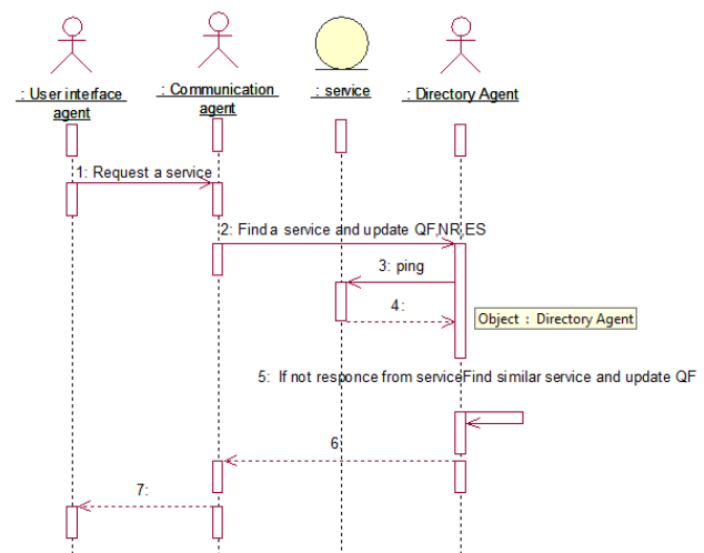
Figure 4: Sequence diagram when user allows a Directory agent to decide which service is best for the application
