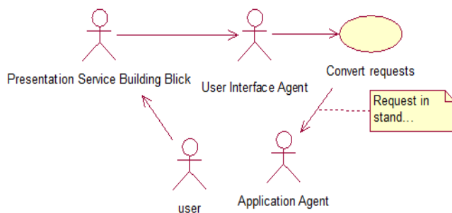
Figure 2: Use case diagram of a user interface agent to manage registration and service discovery
