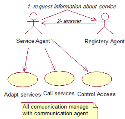
Figure 5: Service agent function, the model proposed
