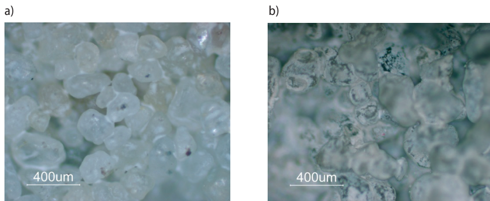
Fig. 2. Morphology of green sand surface I: a) before liquid metal pouring; b) after liquid metal pouring
