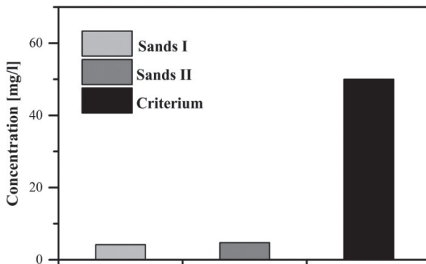
Fig. 4. Comparison of nitrate(V) concentration results
