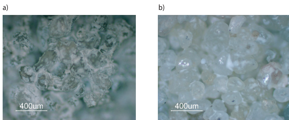
Fig. 3. Morphology of green sand surface II: a) before liquid metal pouring; b) after liquid metal pouring
