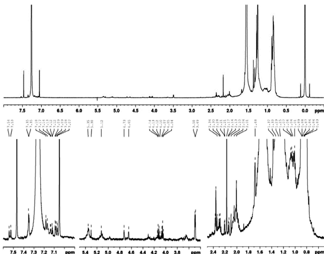
Fig. 5 — 1 H NMR Spectrum of the Peloid Sample.
