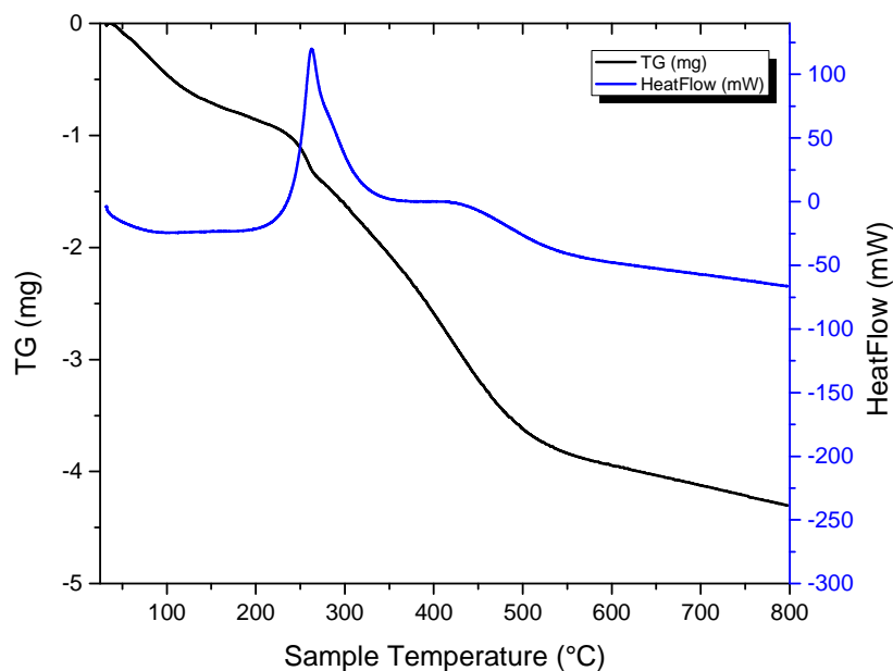
Figure 2. TG-DTA diagram of m-PSZ material.
