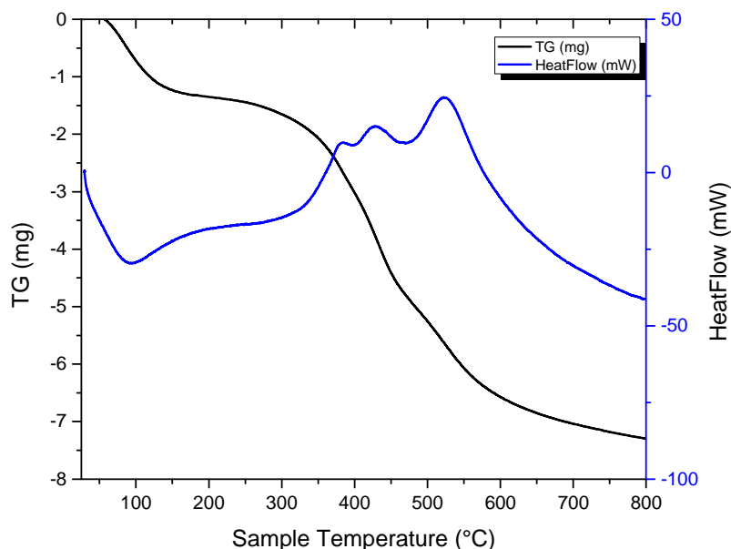
Figure 1. TG-DTA diagram of m-PZ material.
