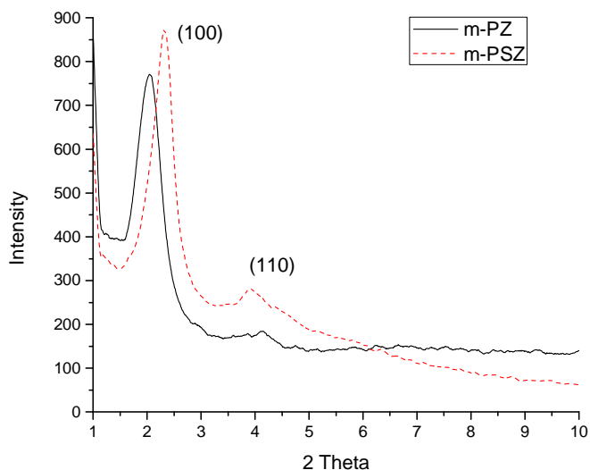
Figure 3. SAXRD patterns of m-PZ and m-PSZ materials.
