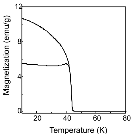
Fig. 5. Magnetization vs. temperature of \text{Mn}_3[\text{Cr}(\text{CN})_6]_2 \cdot n\text{H}_2\text{O} nanoparticle.
