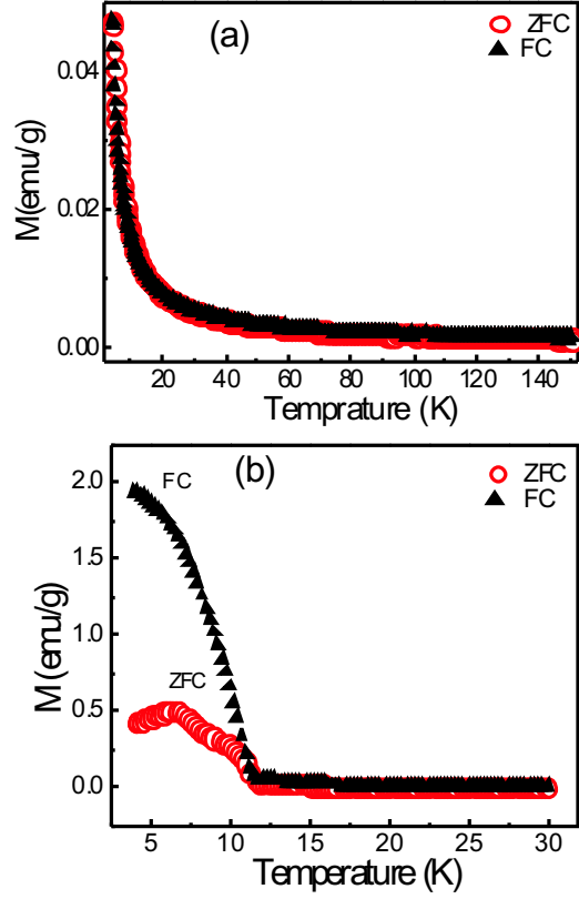
Fig. 4. FC and ZFC vs. temperature of the \text{Rb}_x\text{Mn}[\text{Fe}(\text{CN})_6] samples used water (a) and formamide (b) solvent.
