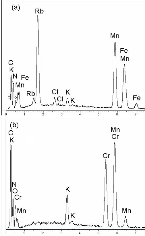
Fig. 3. EDX spectra of \text{Rb}_x\text{Mn}[\text{Fe}(\text{CN})_6] and \text{Mn}_3[\text{Cr}(\text{CN})_6]_2 Prussian blue. For clarity, we show spectra of only samples with formamide.
