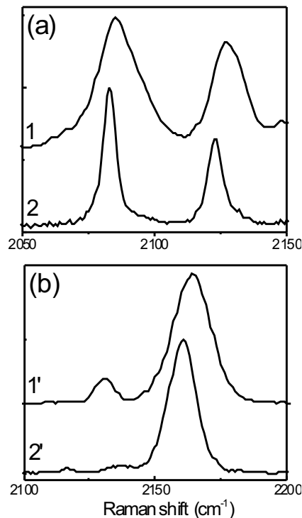
Fig. 6. Raman spectra of (a) \text{Rb}_x\text{Mn}[\text{Fe}(\text{CN})_6] and (b) \text{Mn}_3[\text{Cr}(\text{CN})_6]_2 \cdot n\text{H}_2\text{O} nanoparticle.
