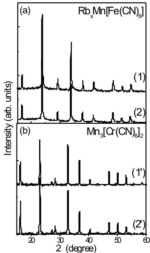
Fig. 2. XRD of (a): \text{Rb}_x\text{Mn}[\text{Fe}(\text{CN})_6] and (b): \text{Mn}_3[\text{Cr}(\text{CN})_6]_2 samples. (1), (1)label for \text{H}_2\text{O} and (2), (2) for formamide solution.
