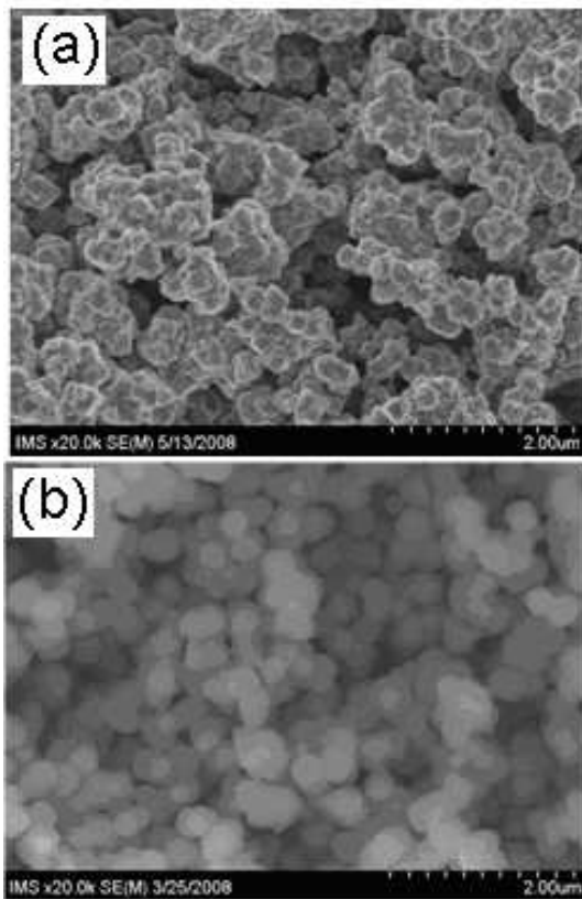
Fig. 1. SEM images of (a) \text{Rb}_x\text{Mn}[\text{Fe}(\text{CN})_6] and (b) \text{Mn}_3[\text{Cr}(\text{CN})_6]_2 . For clarity, we show only image of sample prepared in formamide solution
