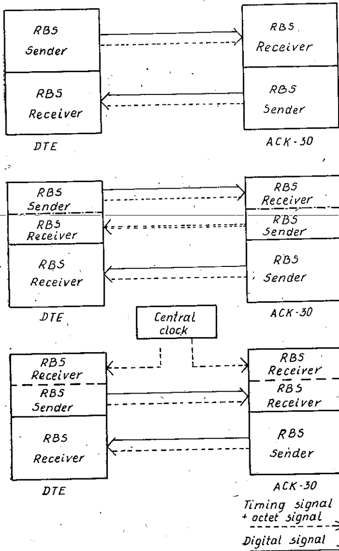
Fig. 3. Digital interfaces a) codirectional; b) contradirectional; c) with central clock
