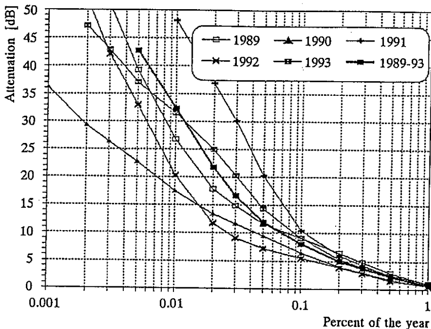
Fig. 3. Annual attenuation distributions in the years 1989-93 at 18.6 GHz and average distribution
