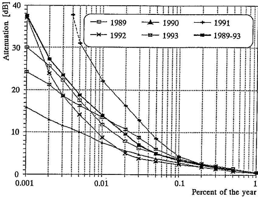
Fig. 2. Annual attenuation distribution in the years 1989-93 at 11.5 GHz and average distribution
