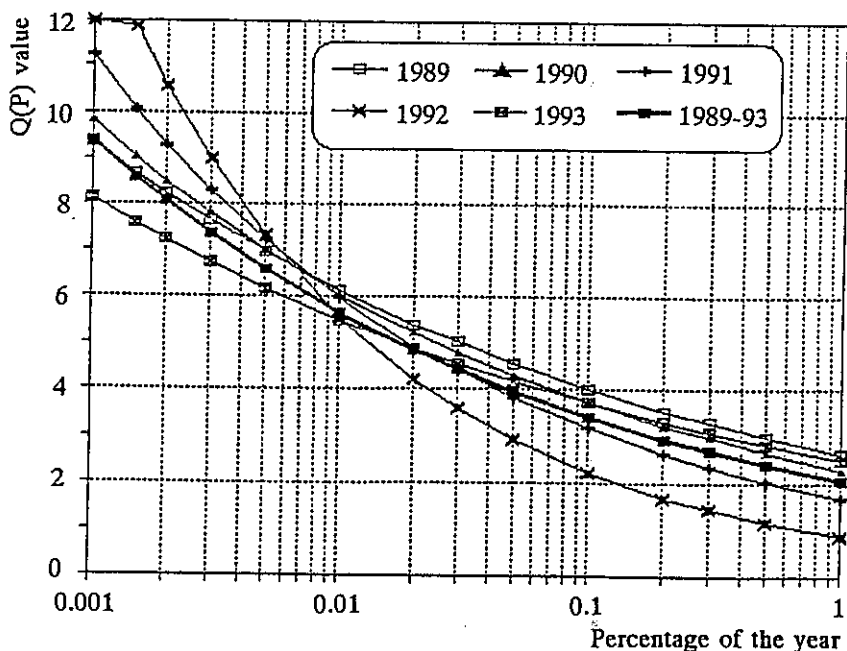
Fig. 5. Q(p) graphs for attenuations distributions at 11.5 GHz in 1989-93
