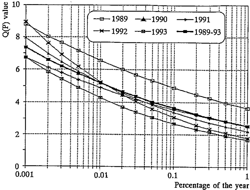
Fig. 4. Q(p) graphs for rain rate distributions in the years 1989-93
