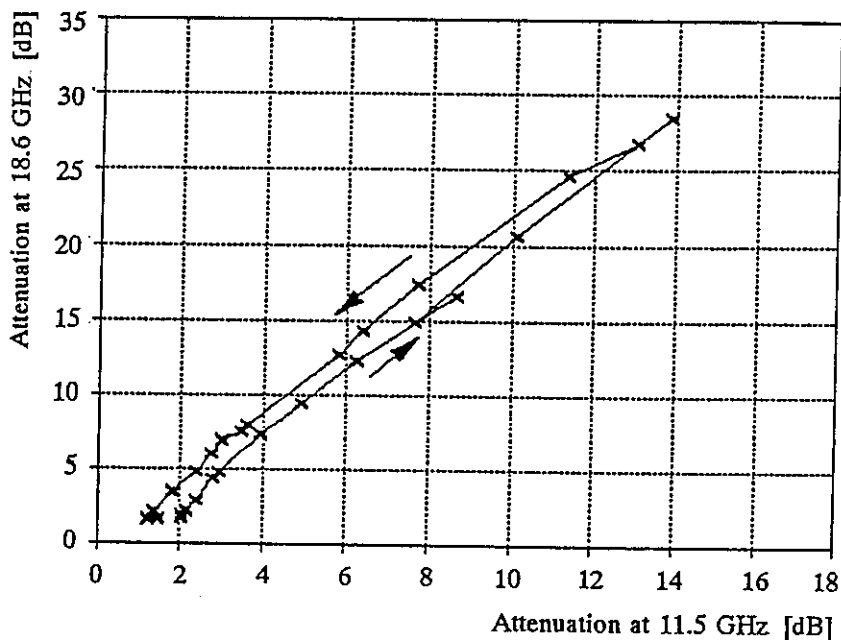
Fig. 1. Attenuation at 18.6 GHz versus attenuation at 11.5 GHz during the passage of the path by rain cell
