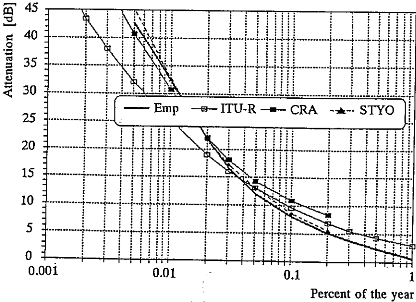
Fig. 12. Empirical and predicted attenuation distributions at 18.6 GHz
