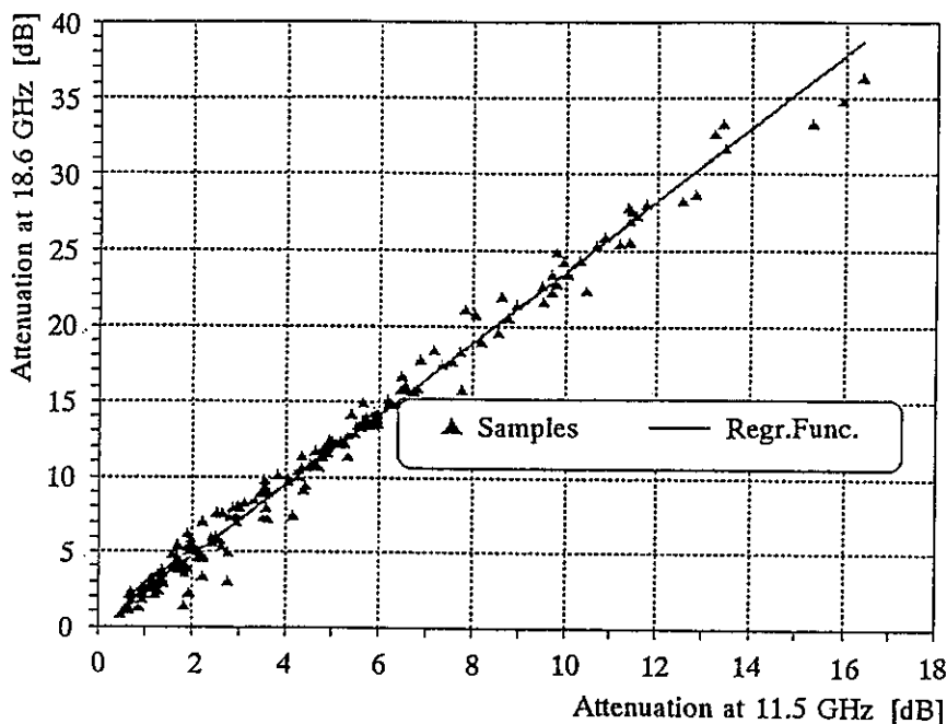
Fig. 9. Regression of attenuation at 18.6 GHz in terms of attenuation at 11.5 GHz
