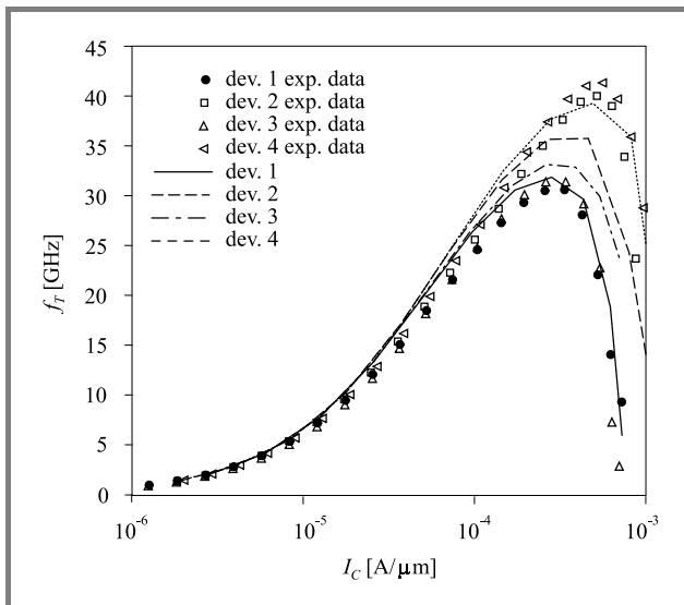
Fig. 13. Frequency f_T versus I_C at V_{CE} = 1.5 V. Comparison between measurement and hydrodynamic simulation with Minimos-NT.
