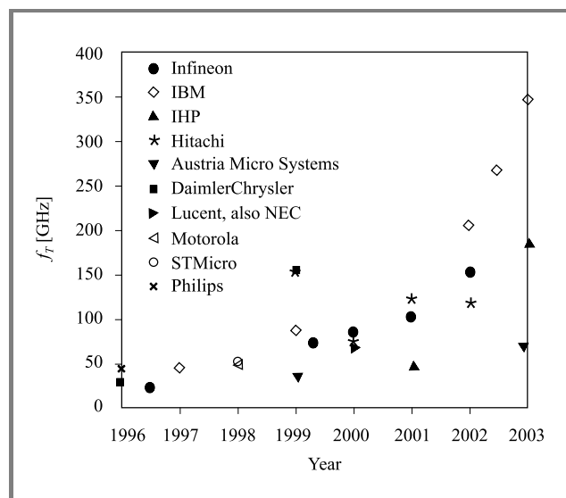
Fig. 1. Current gain cutoff frequency f_T of SiGe HBTs over time.
