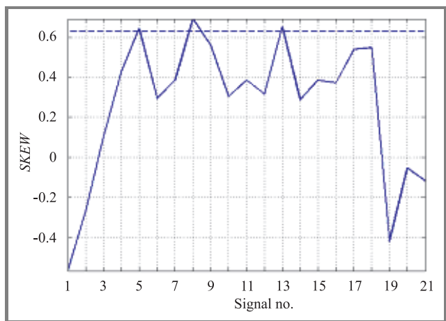
Fig. 3. Skewness.
