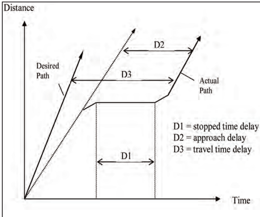
Figure 4: Illustration of Intersection Delays
