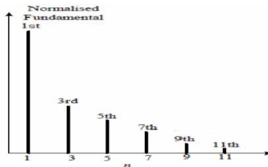
Figure 4 : Harmonic Spectra of an Inverter
