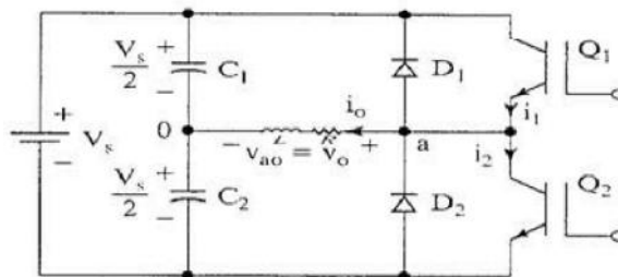
Figure 2 : Circuit Diagram of Single Phase Half Bridge Inverter
