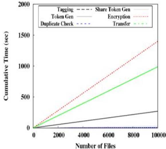
Figure 3 Time Break Down For Different Number Of Files
