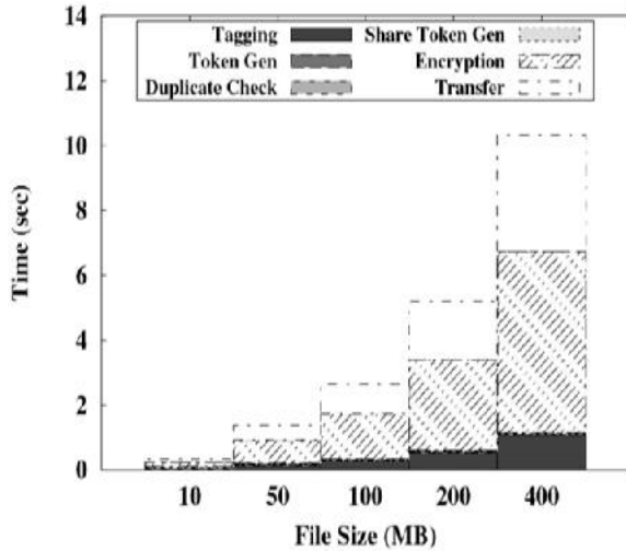
Figure 2 Time Breakdown For Different File Size Number of Stored Files
