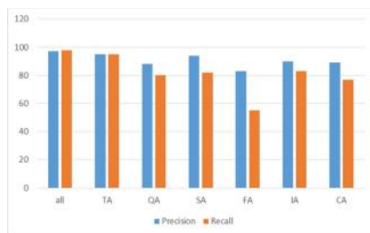
Fig 4. Performance of Basic Annotator
