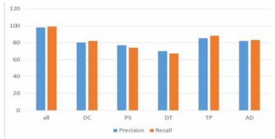
Fig 3. Performance of Alignment Features
