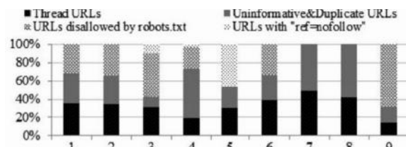
Fig- 2. Ratio of different URLs discovered by a generic crawler
