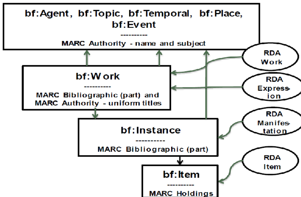
Figure 1: BIBFRAME data model with MARC and RDA mapping
