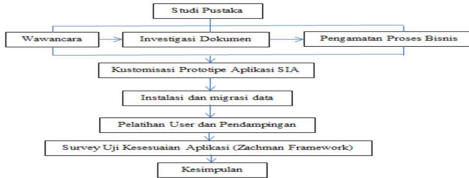
Gambar 2: Tahapan Penelitian
