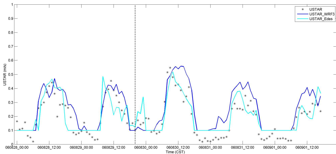
Figure 13. Time series for friction velocity for observations (stars), WRF (dark blue line), and MM5 (light blue line)
