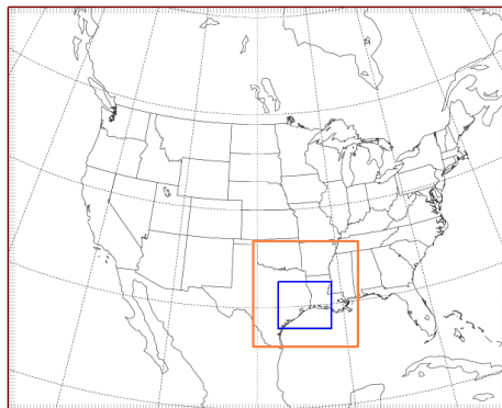
Figure 3. Nesting domain for WRF model, where the blue box is the 4-km domain that all model outputs were extracted from
