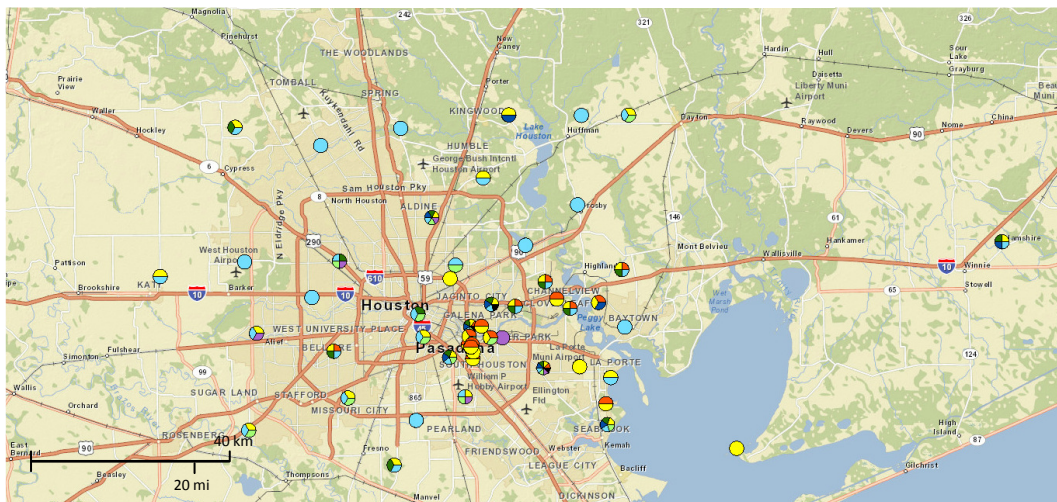
Figure 2. TCEQ CAMS sites for the modeling region
