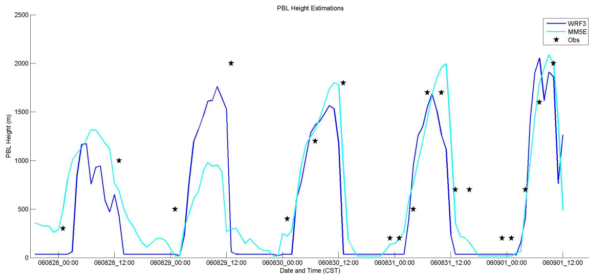
Figure 14. Time series of PBL height for the study period for observations (stars), WRF (dark blue line), and MM5 (light blue line)
