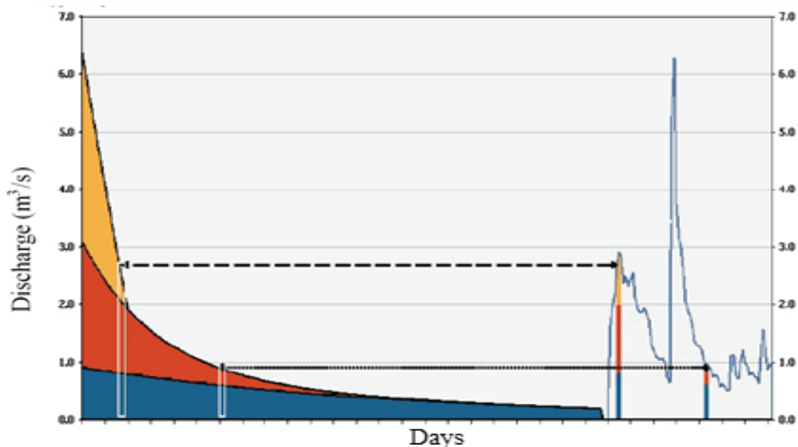
Figure 2. Principles of hydrograph separation based on the master RC [3]
