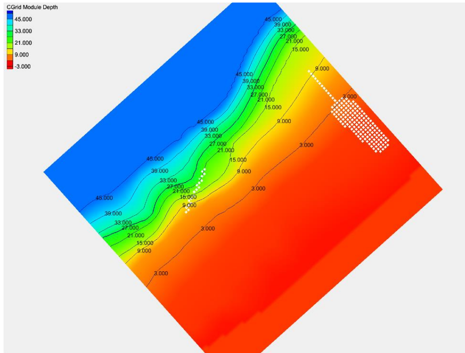
Figure 7. Numerical model bathymetry grid for 2D wave model of Waikelo Port
