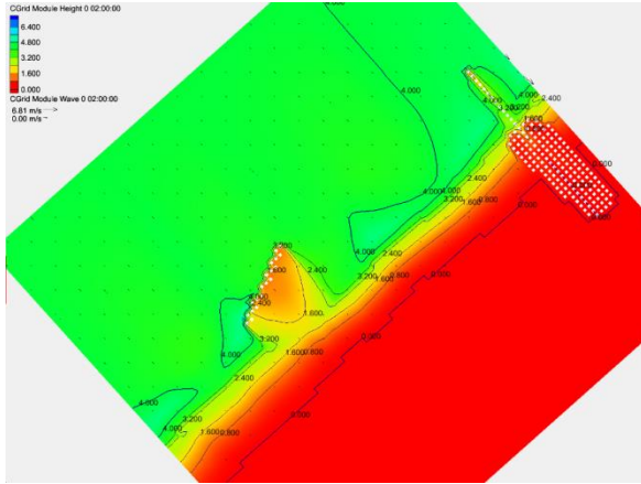
Figure 9. Simulated wave propagation due to 4.0m of significant wave height ( H_s ).
