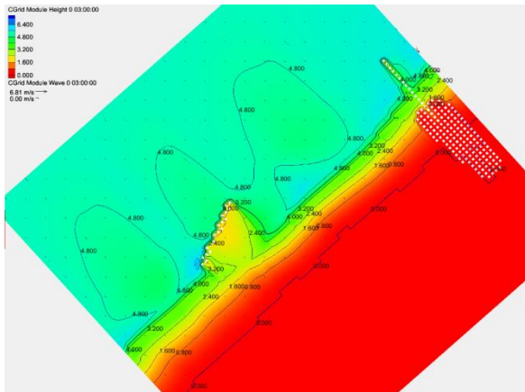
Figure 11. Simulated wave propagation due to 5.0m of significant wave height ( H_s ).
