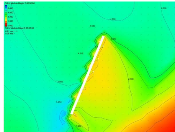
Figure 12. Distribution of wave height in surround breakwater due to H_s = 5.0m .
