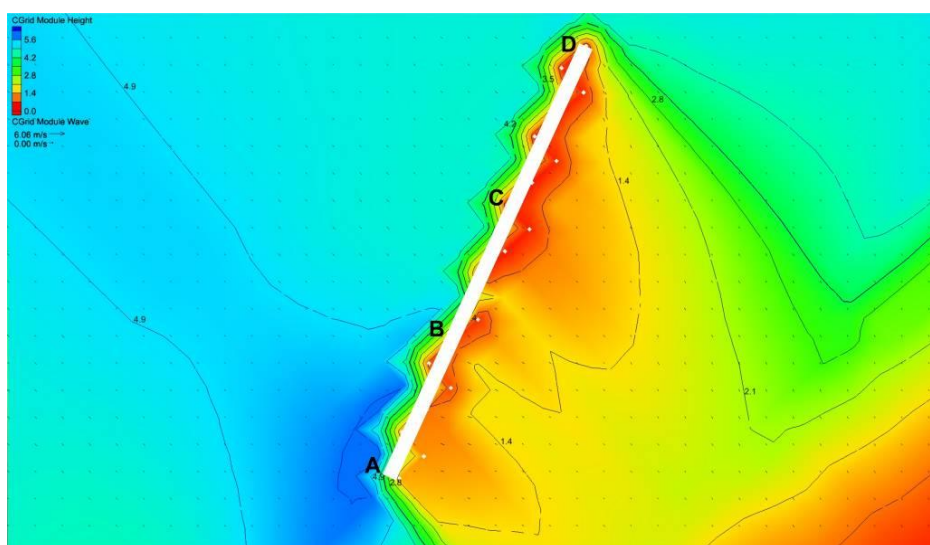
Figure 8. Examination points (A, B, C, D) of 2D wave model simulation in surround breakwater
