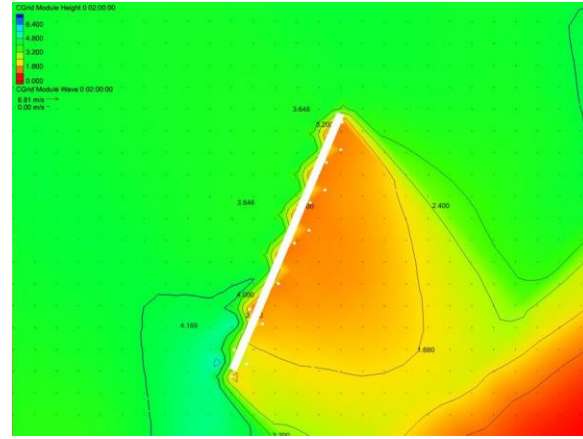
Figure 10. Distribution of wave height in surround breakwater due to H_s = 4.0m .
