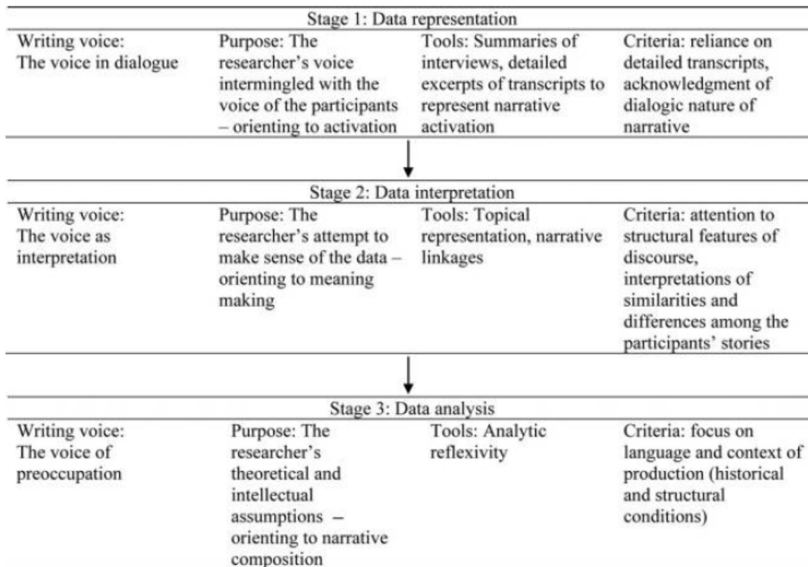
Figure 1. Data analysis
