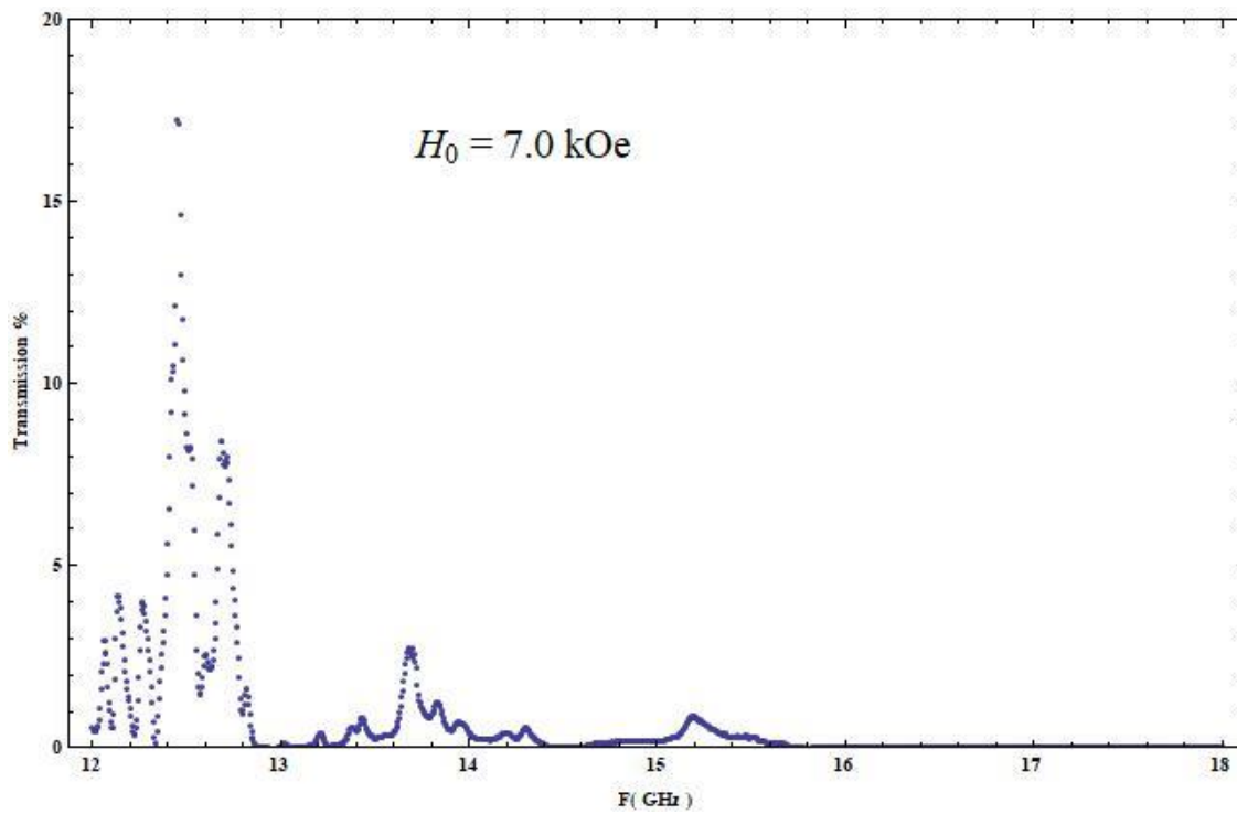
Fig. 4.7.79 Transmission vs. Frequency for H_0 = 7.0 \text{ kOe}
