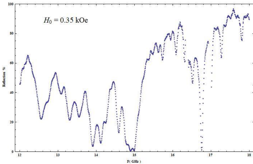
Fig. 4.7.20 Reflection vs. Frequency for H_0 = 0.35 kOe
