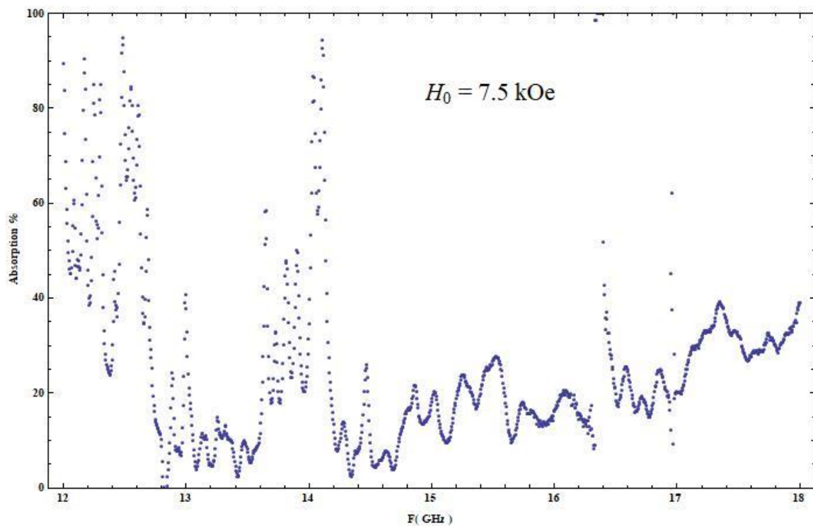
Fig. 4.7.84 Absorption vs. Frequency for H_0 = 7.5 \text{ kOe}
