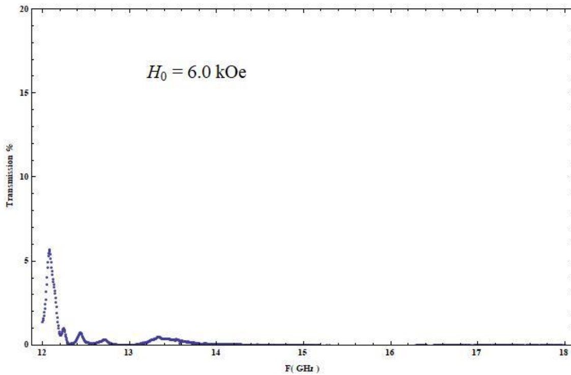
Fig. 4.7.73 Transmission vs. Frequency for H_0 = 6.0 \text{ kOe}
