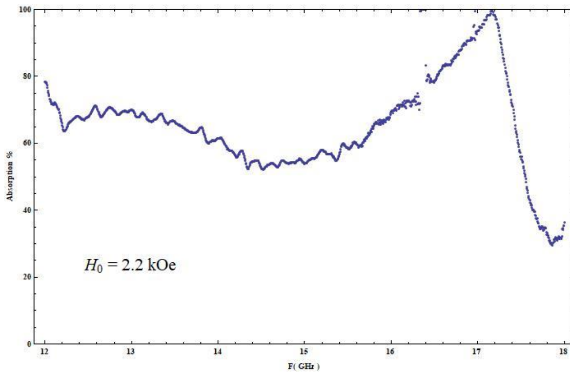
Fig. 4.7.60 Absorption vs. Frequency for H_0 = 2.2 kOe
