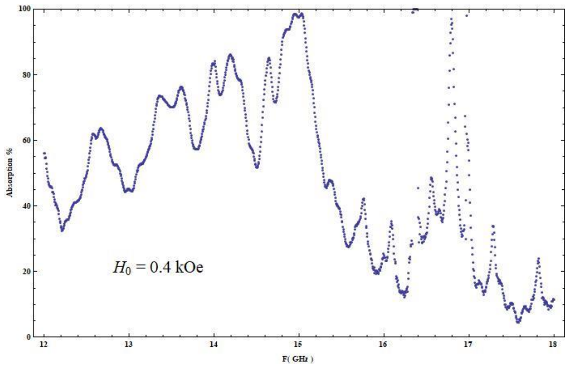
Fig. 4.7.24 Absorption vs. Frequency for H_0 = 0.4 \text{ kOe}
