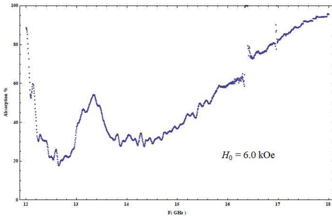
Fig. 4.7.75 Absorption vs. Frequency for H_0 = 6.0 kOe
