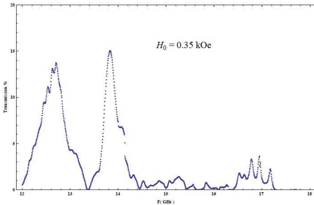
Fig. 4.7.19 Transmission vs. Frequency for H_0 = 0.35 kOe
