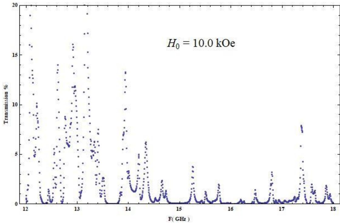
Fig. 4.7.97 Transmission vs. Frequency for H_0 = 10.0 \text{ kOe}
