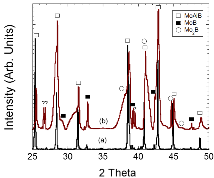
Figure 3.1: XRD plot of, (a) MoAlB, and (b) etched MoAlB particulates.
