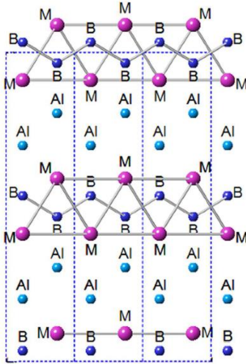
Figure 1.2: Crystal structure of MoAlB [17].
