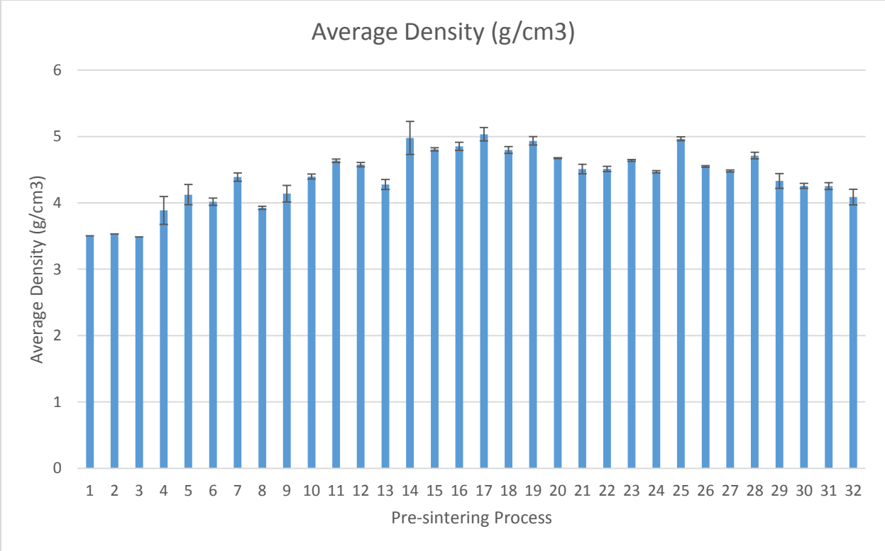
Figure 5.1: Average densities (g/cm 3 ) of various pressureless sintered compacts.
