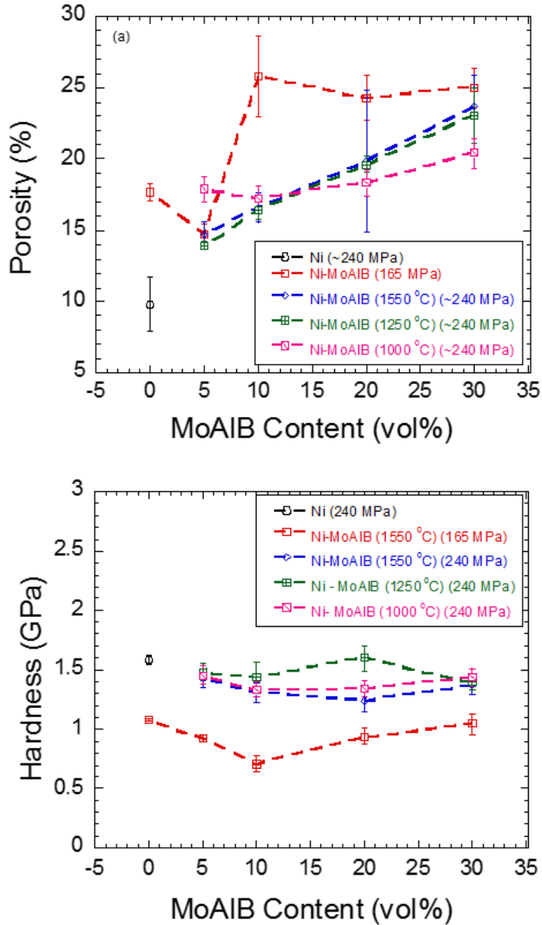
Figure 4.4: Plot of, (a) porosity, and (b) hardness versus MoAIB content in Ni-matrix.
