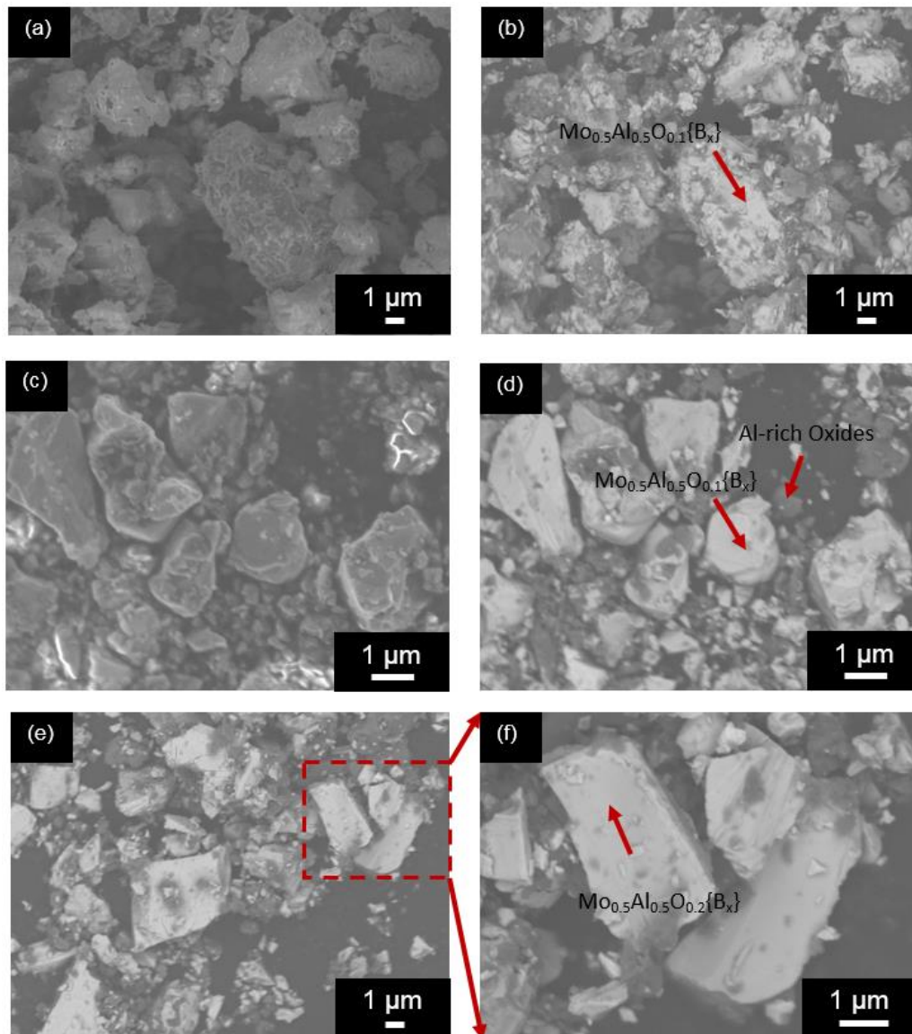
Figure 4.1: FESEM micrographs of MoAlB particles synthesized at, (a) 1000 °C in SE, (b) BSE of the same region, (c) 1250 °C in SE, (d) BSE of the same region, (e) 1550 °C in BSE, and (f) BSE at higher magnification.
