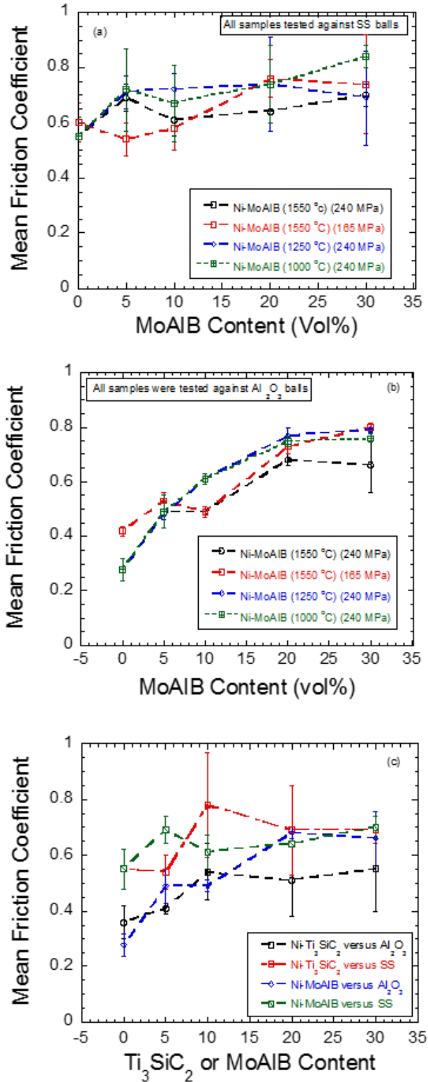
Figure 4.6: Plot of mean friction coefficient ( \mu_{\text{mean}} ) versus MoAIB content during sliding against, (a) SS, and (b) alumina balls, and (c) comparison of \mu_{\text{mean}} of Ni-Ti 3 SiC 2 [13] or Ni-MoAIB (1550 °C) against SS and Al 2 O 3 balls, respectively.
