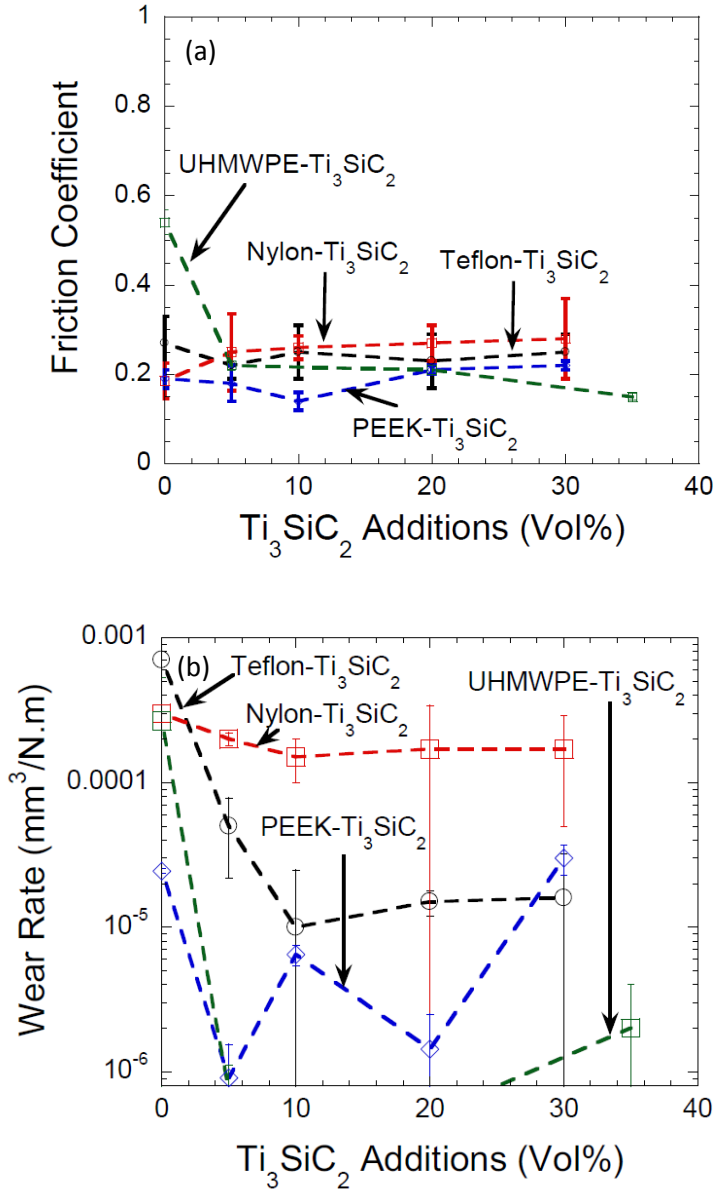
Figure 1.5: Plot of MRPs (a) \mu_m and (b) wear rates as a function of Ti_3SiC_2 content [26].
