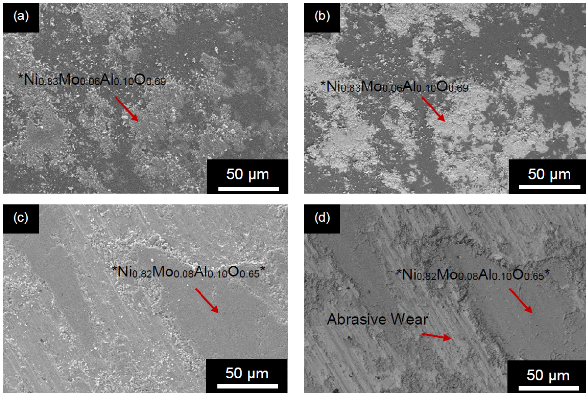
Figure 4.10: SEM micrographs of alumina surface in, (a) SE, (b) BSE, and corresponding Ni-30%MoAlB (1550 °C) surface in, (c) SE, and (d) BSE during dry sliding.
