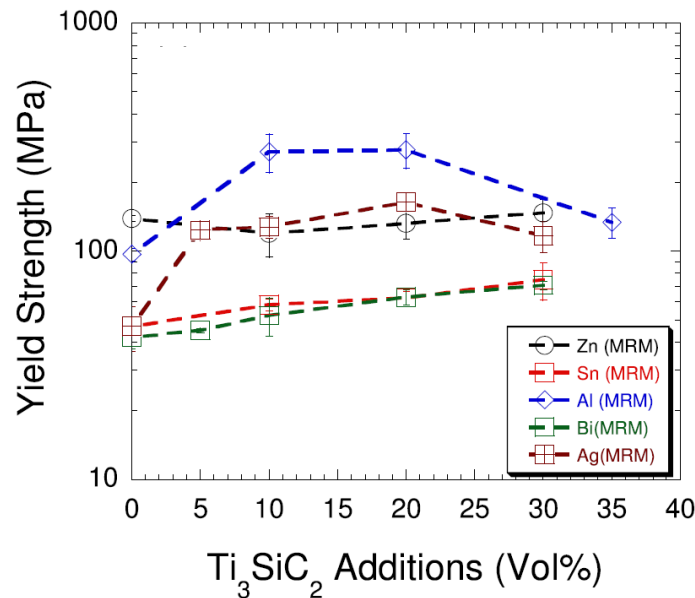
Figure 1.3: Plot of stress versus displacement of yield strength of different MRMs versus Ti_3SiC_2 content [22].
