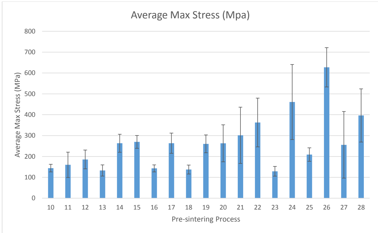
Figure 5.3: Average maximum stresses (MPa) of various pressureless sintered compacts.
