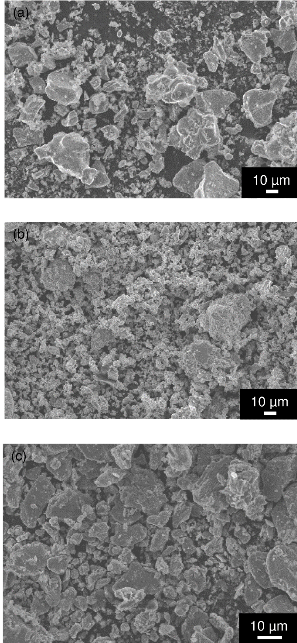
Figure 2.5: SE SEM micrographs of synthesized powders of, (a) Cr 2 AlC, (b) Cr 2 GaC, and (c) V 2 AlC.
