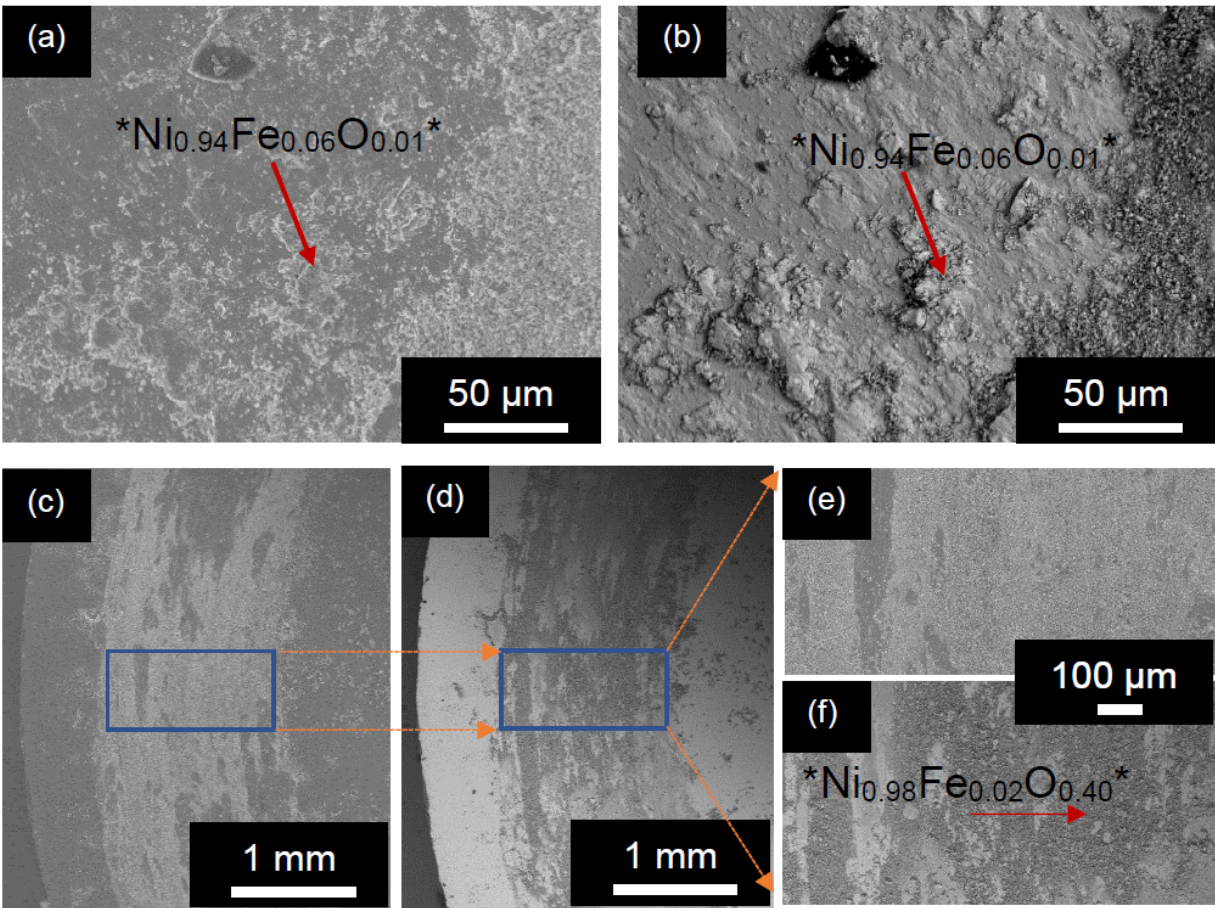
Figure 4.8: SEM micrographs of SS surface in, (a) SE, (b) BSE, and corresponding Ni surface in, (c) SE, (d) BSE, and higher magnification of the region marked in (d) in, (e) SE and (f) BSE during dry sliding.
