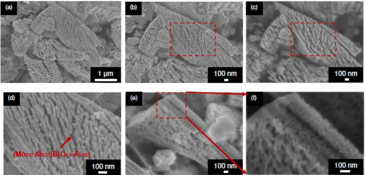
Figure 3.3: FESEM SE micrographs of, (a) etched MoAlB particulates, (b) top surface of etched MoAlB particulate at higher magnification, (c) BSE of the same region, (d) higher magnification of the marked region in (b), (e) side view of an etched particulate, and (f) higher magnification of the same region.
