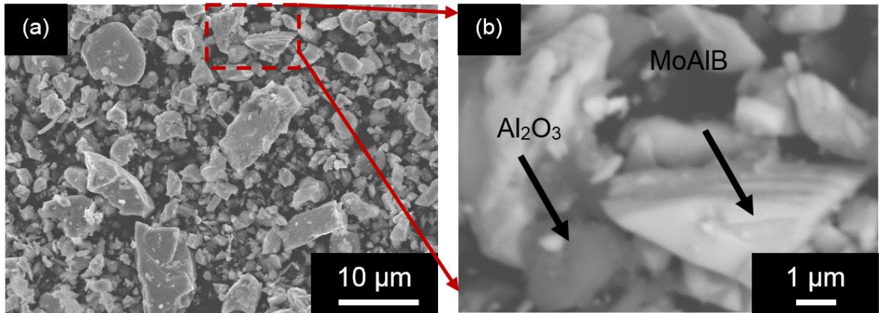
Figure 3.2: SEM SE micrograph of as-synthesized MoAlB particulates at, (a) lower, and (b) BSE image at higher magnifications.
