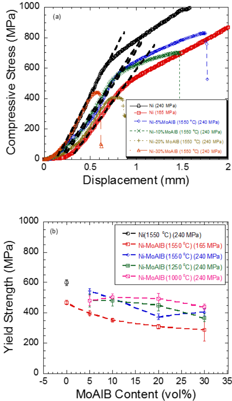
Figure 4.5: Plot of, (a) compressive stress versus displacement, and (b) yield strength versus MoAlB content.
