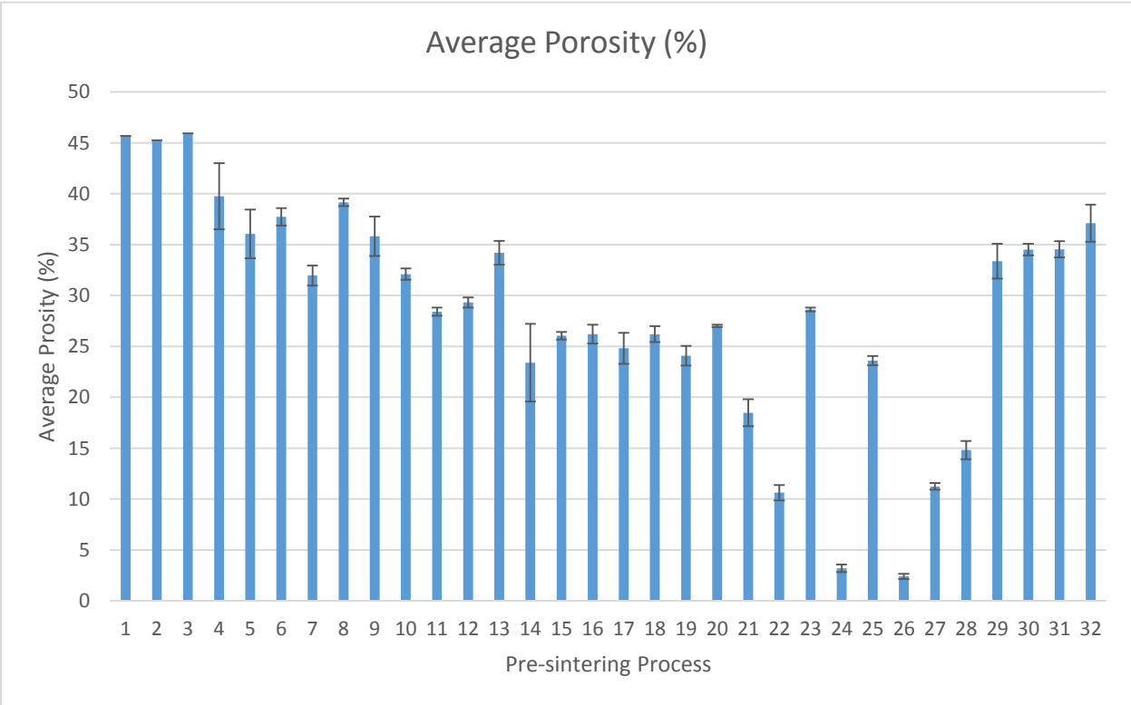
Figure 5.2: Average porosities (%) of various pressureless sintered compacts.
