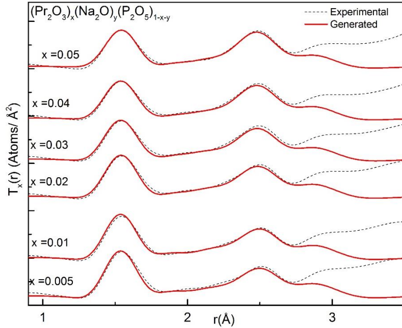
Figure 4.14 (a) : T(r) profile of for (\text{RE}_2\text{O}_3)_x(\text{Na}_2\text{O})_y(\text{P}_2\text{O}_5)_{1-x-y} glasses, continue next page.
