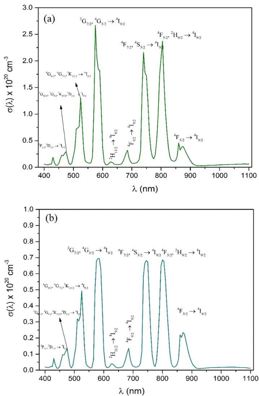
Figure 4. 21 : Absorption Cross Section of Nd^{3+} -doped sodium phosphate glasses (a) x = 0.092 molar fraction with concentration of Nd^{3+} N = 2.90 \times 10^{20} \frac{\text{ions}}{\text{cm}^3} (b) x = 0.03 molar fraction
