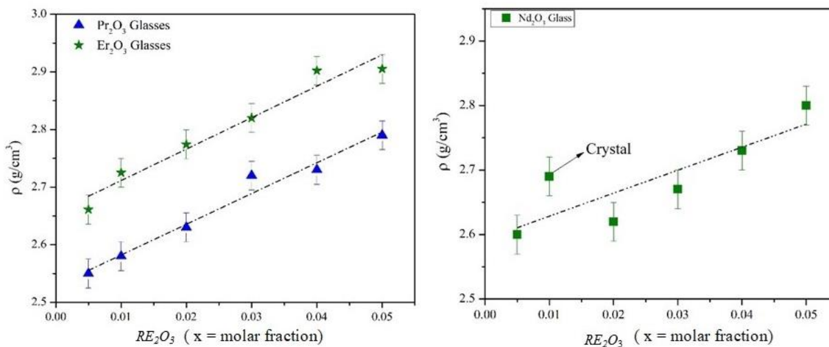
Figure 4. 1: Dependence of the density of Pr, Er and Nd doped sodium phosphate glasses on \text{RE}_2\text{O}_3 concentration with error bars at \pm 0.03 \text{ g/cm}^3 .
