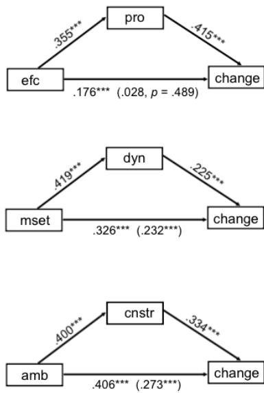
Figure 15. Indirect Effects
