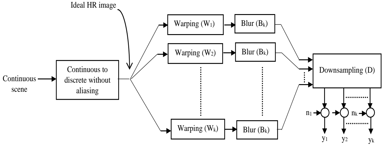
Figure 3.2: Observation model relating LR image with HR image.
