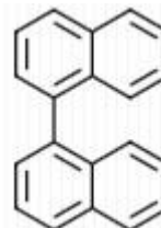
4,4'-binaphthalene
