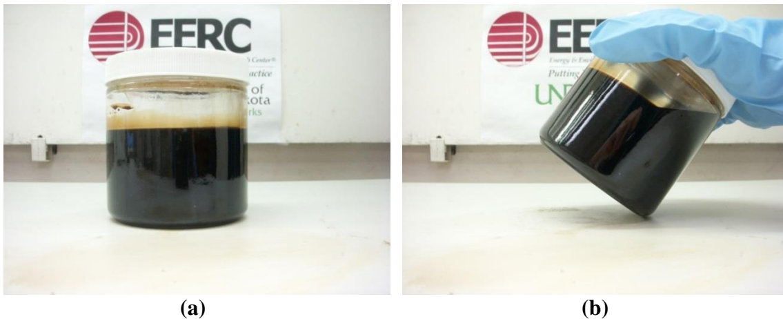
Figure 7-83. Lo-pour fuel oil – crude jatropha oil blend, cooled from 220°F to 75°F. (a) shows the blend sitting flat, and (b) shows the blend tilted at an angle.
