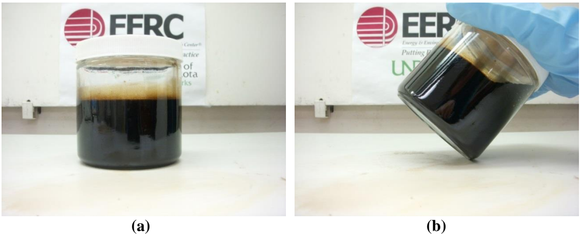
Figure 7-82. Lo-pour fuel oil – crude palm oil blend, cooled from 220°F to 75°F. (a) shows the blend sitting flat, and (b) shows the blend tilted at an angle.
