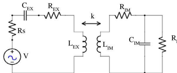
Figure 4. A simplified circuit diagram for the inductive link with matching capacitors. Reproduced courtesy of The Electromagnetics Academy.
