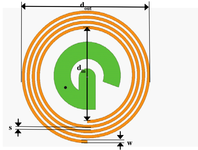
Figure 3. Geometrical parameters of a circular planar spiral coil. Reproduced courtesy of The Electromagnetics Academy.
