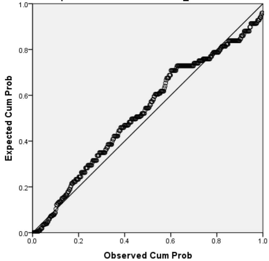
Figure 3. Normal P.P Plot (probability plot) regression on intrinsic motivation
