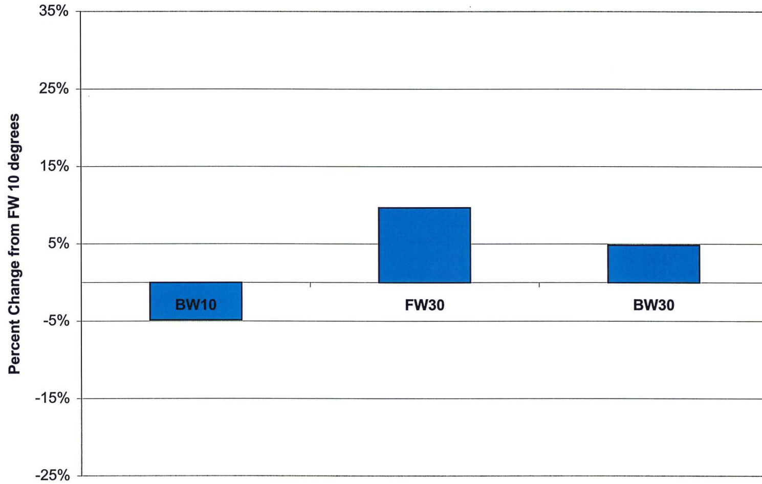
Figure 5. EMG activity in the semitendinosus muscle during the experimental trials.
