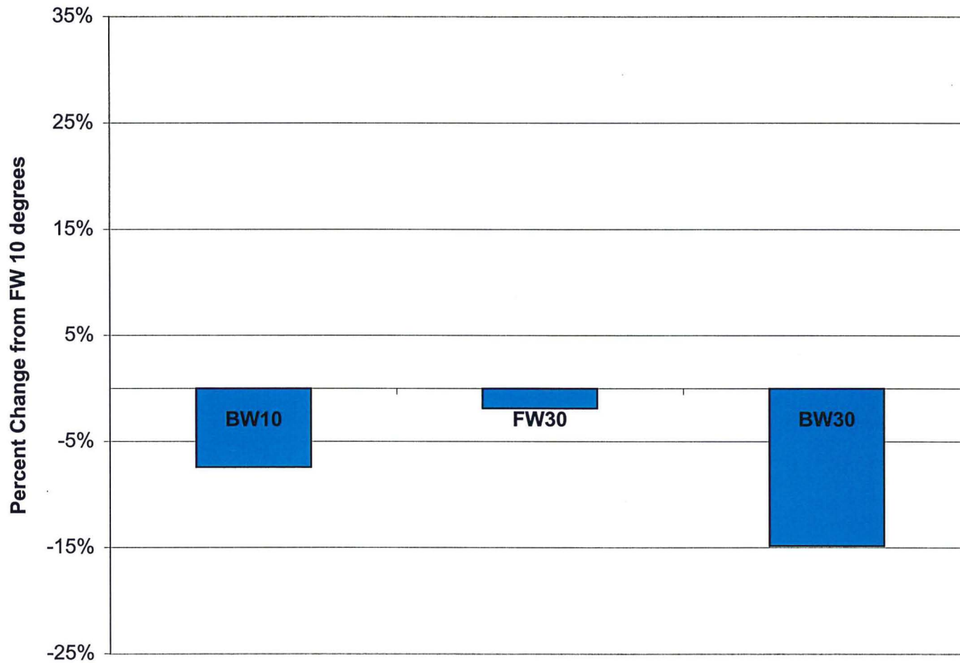
Figure 10. EMG activity in the anterior tibialis muscle during the experimental trials.
