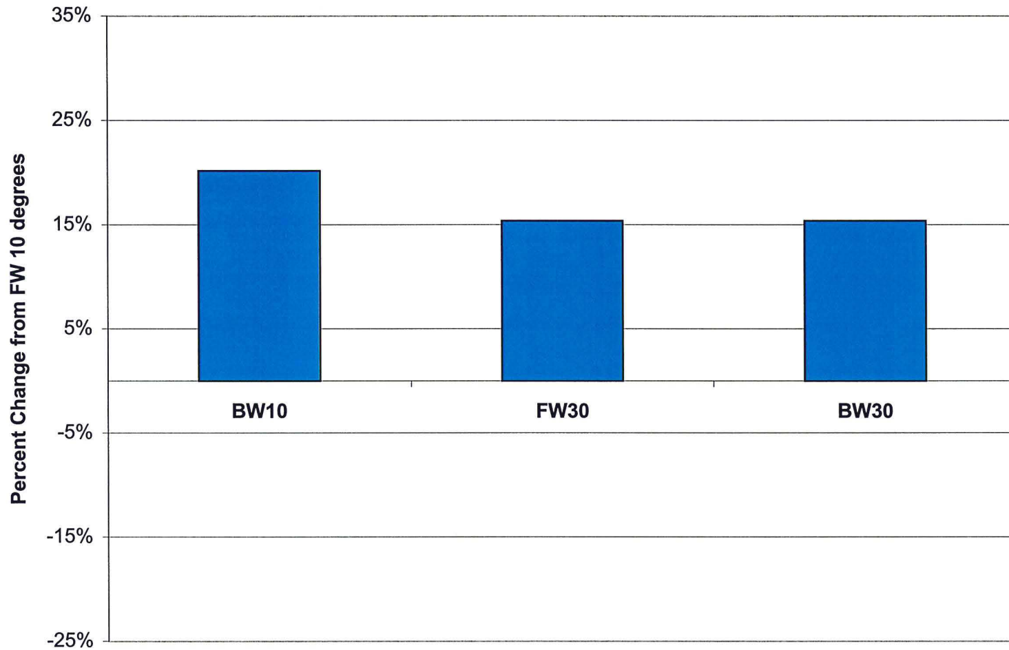
Figure 8. EMG activity in the vastus medialis muscle during the experimental trials.
