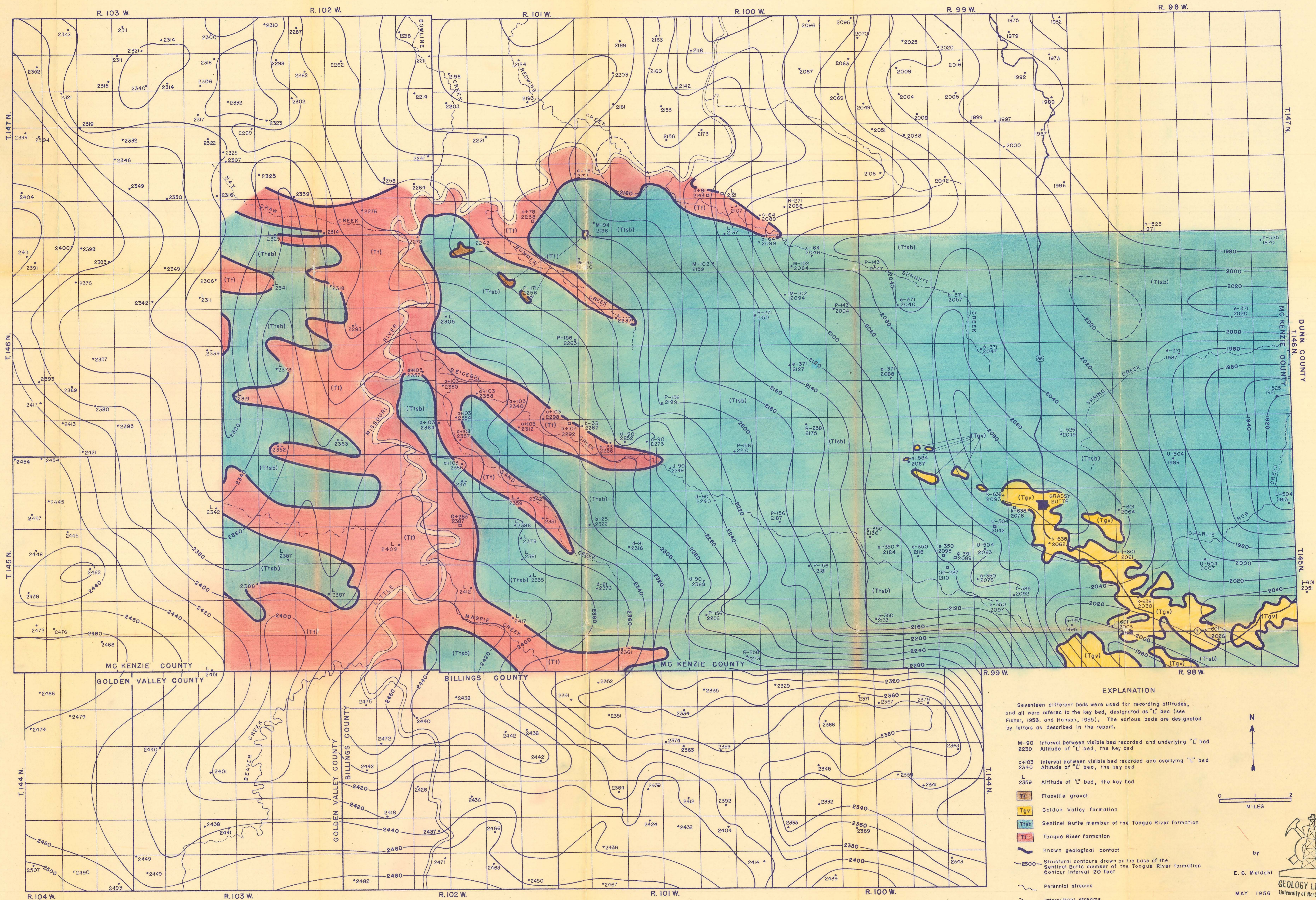
GEOLOGIC MAP OF THE GRASSY BUTTE AREA, MCKENZIE COUNTY, NORTH DAKOTA STRUCTURAL CONTOURS AT THE BASE OF THE SENTINEL BUTTE MEMBER OF THE TONGUE RIVER FORMATION
