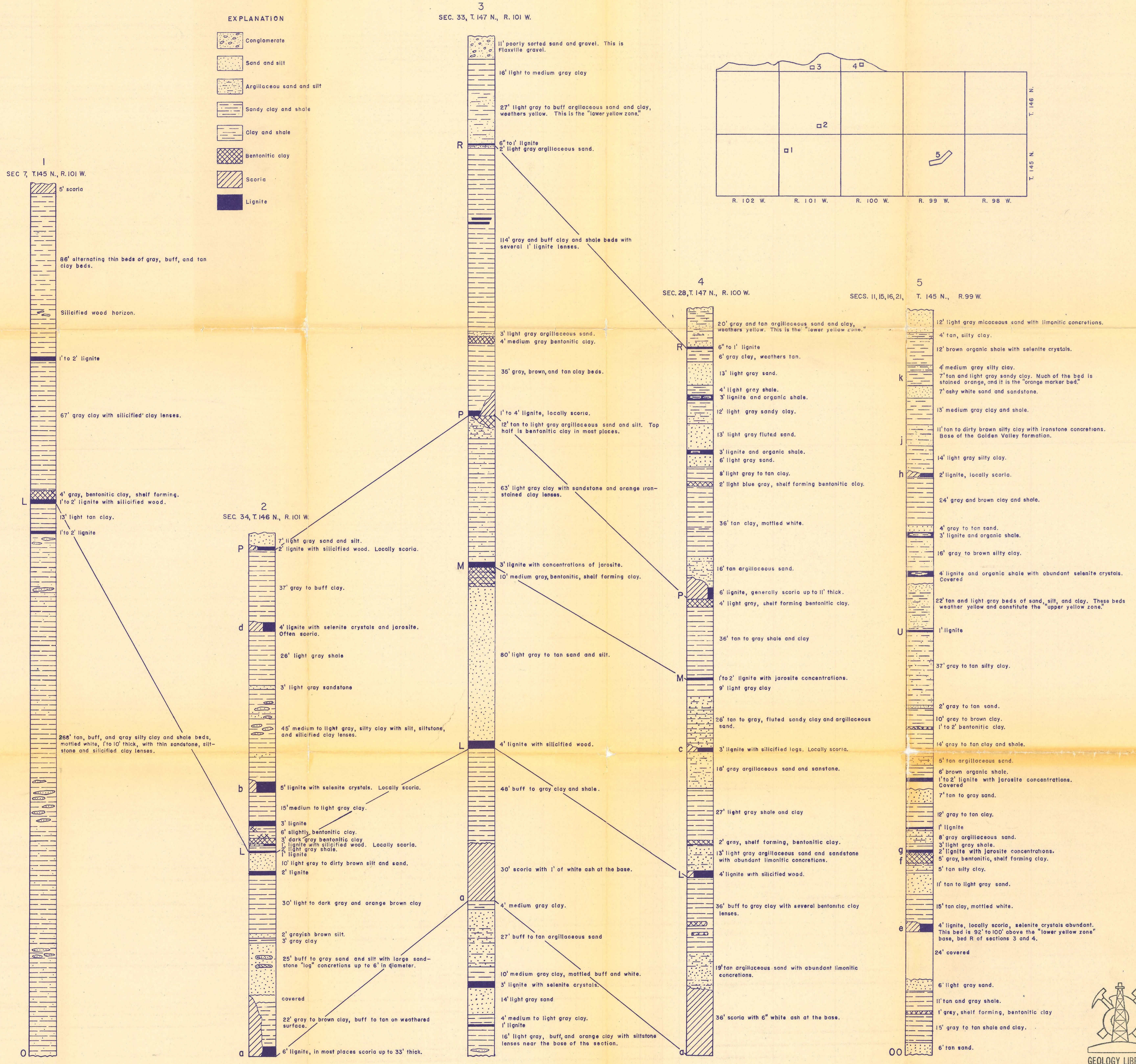
STRATIGRAPHIC SECTIONS GRASSY BUTTE AREA
